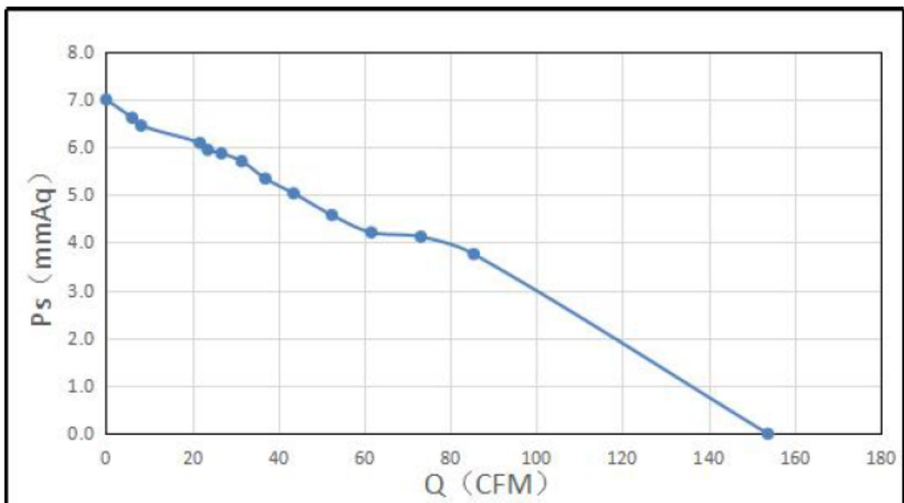
P-Q Curve
