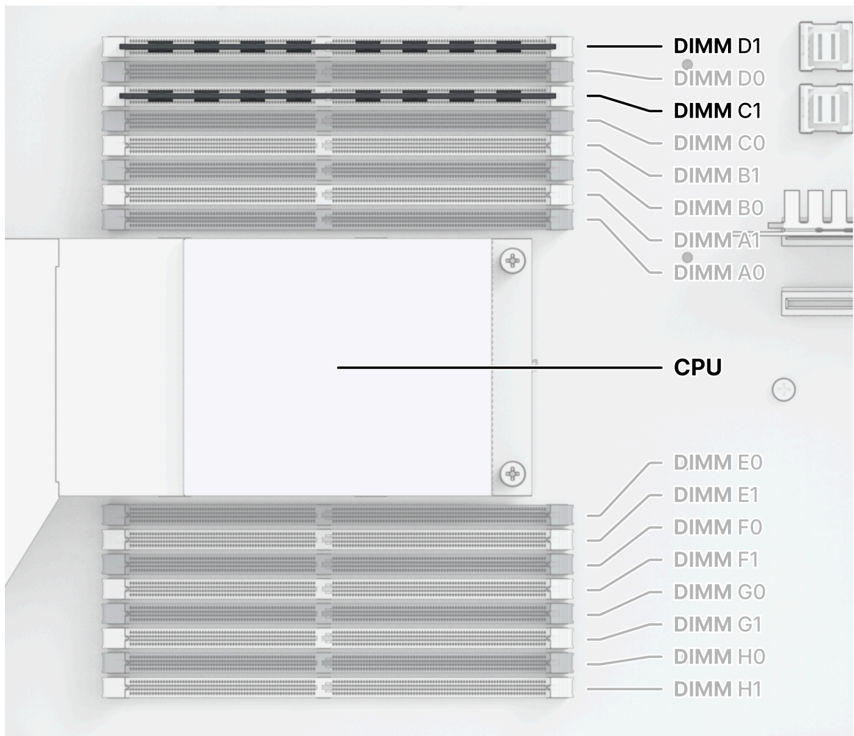
4. Example 2: 4 DIMM Population
