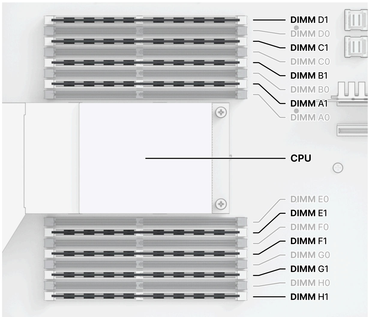
6. Example 4: 16 DIMM Population
