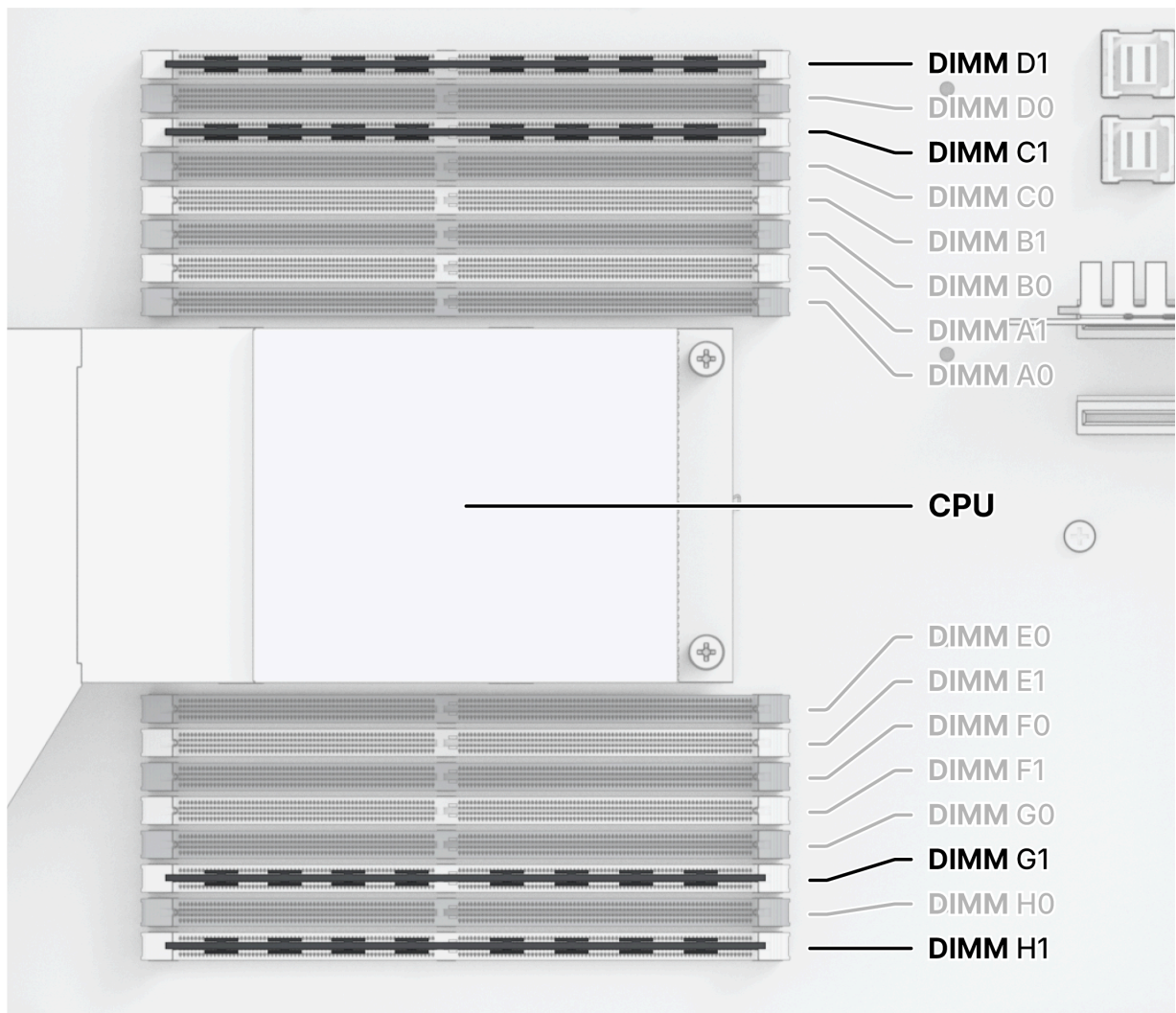
5. Example 3: 8 DIMM Population
