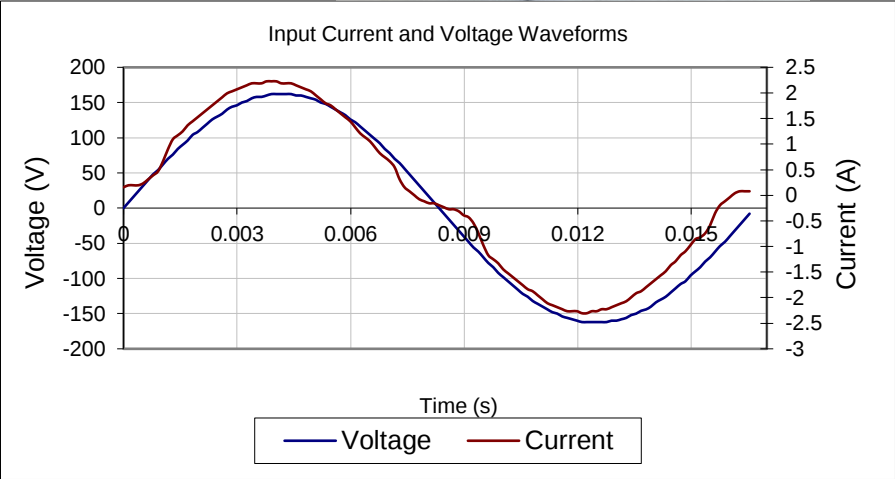
Input AC Current Waveform (ITHD = 10.85%, 50% Load)
