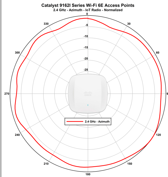
Figure 15: CW9162I - IoT Antenna-Normalized Radiation Pattern (2.4-GHz Azimuth)
