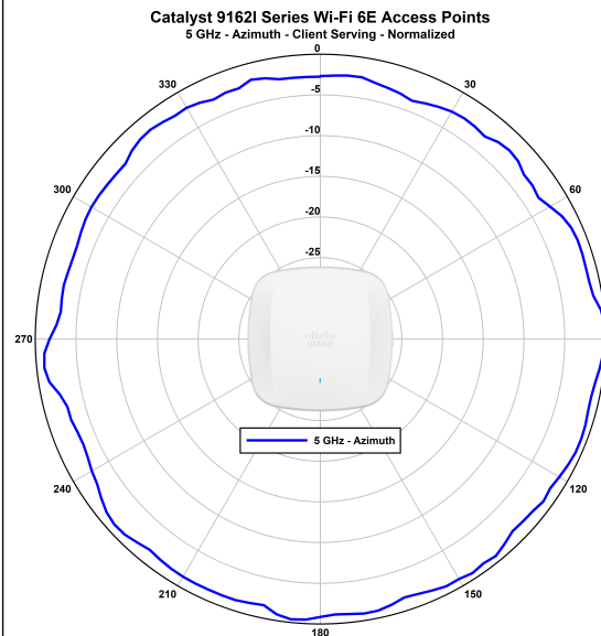
Figure 5: CW9162I - Client-Serving Normalized Radiation Pattern (5-GHz Azimuth)
