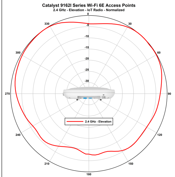
Figure 16: CW9162I - IoT Antenna-Normalized Radiation Pattern (2.4-GHz Elevation)
