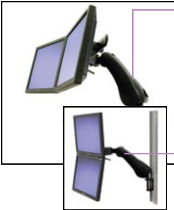
HD Dual-Monitor Arm crossbar tilts monitors up 25° and down 10° using small lever behind monitors. Maximum monitor width is 23¼" (590 mm).
