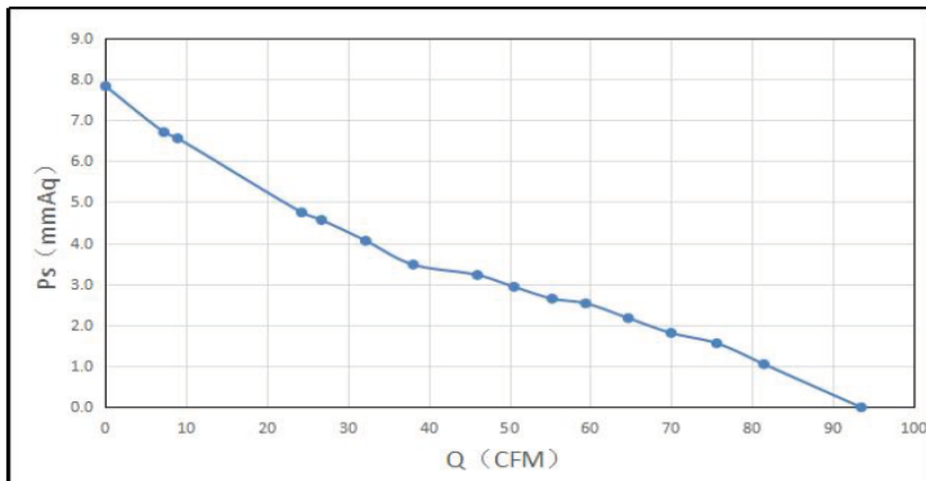
P-Q Curve
