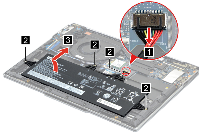
Figure 4. Remove the battery pack
