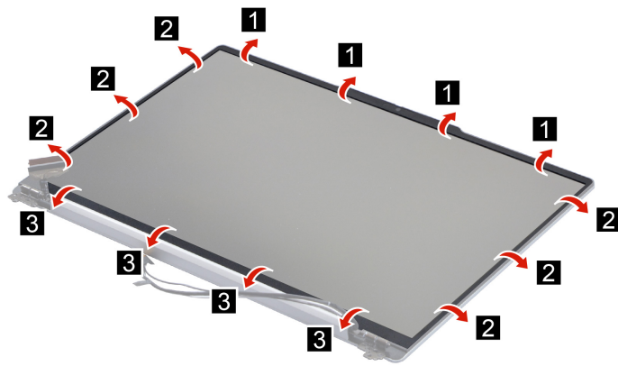
Figure 29. Remove the panel bezel
