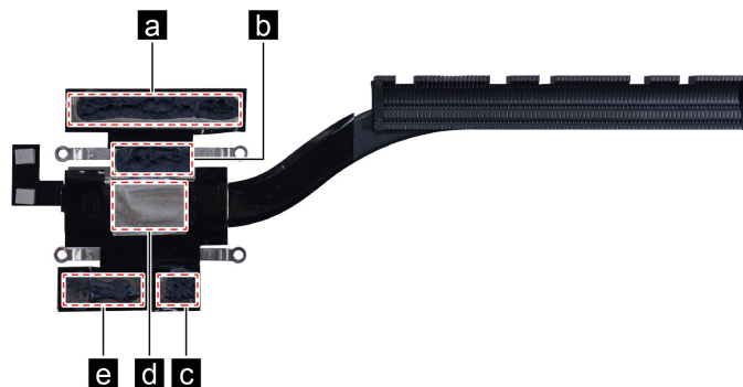
Figure 14. Areas on the heat sink where thermal interface materials should be applied
