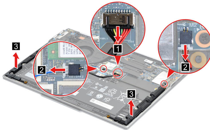
Figure 9. Remove the speakers
