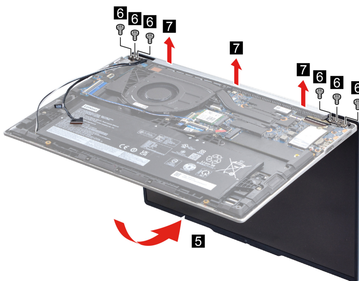
Figure 27. Remove the display assembly
