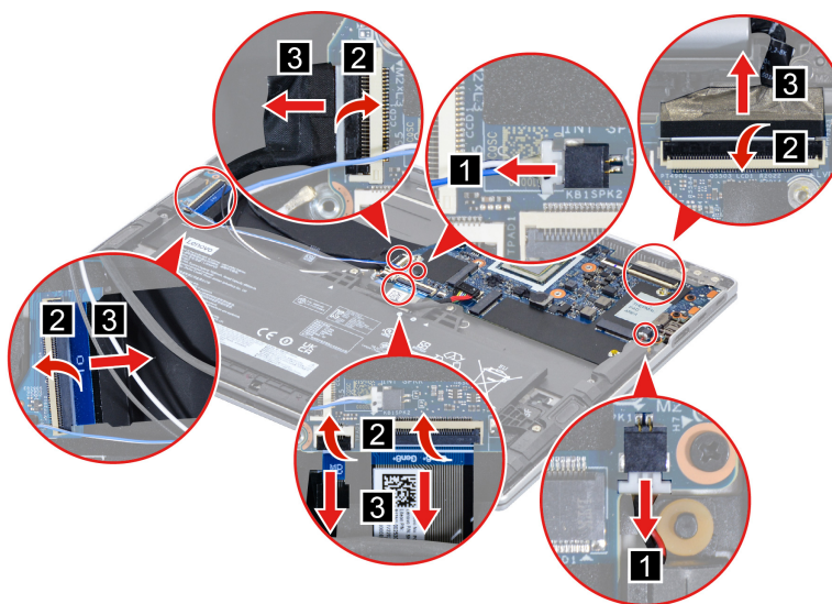
Figure 23. Disconnect cables connected to the system board and disconnect the I/O board cable
