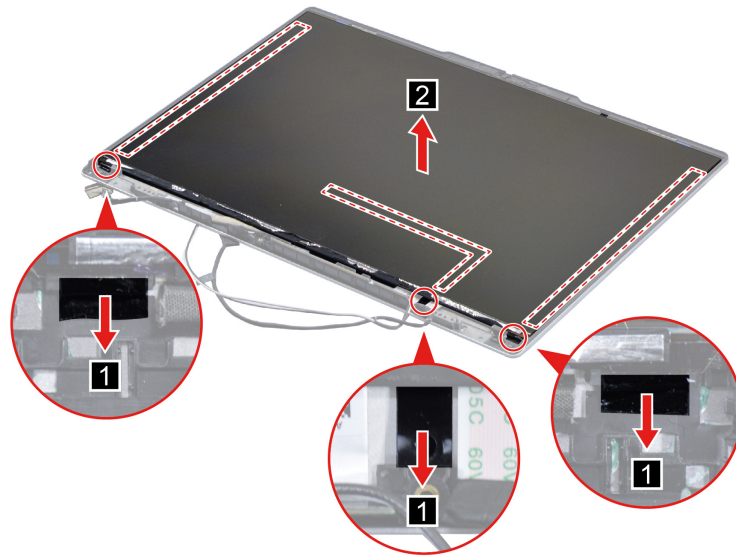
Figure 32. Remove the panel
