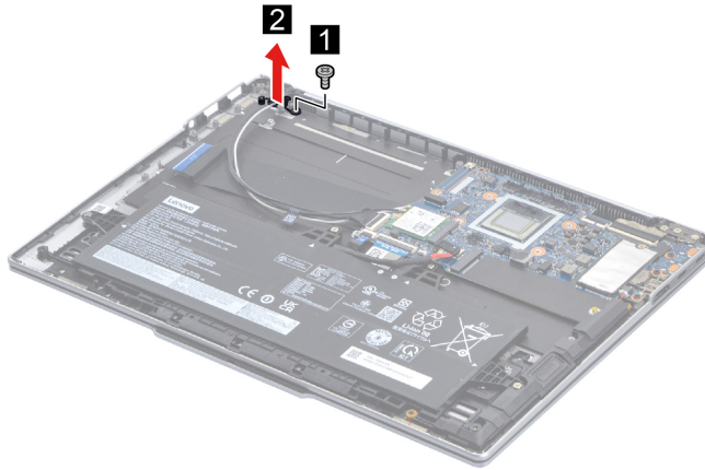
Figure 20. Remove the power button
