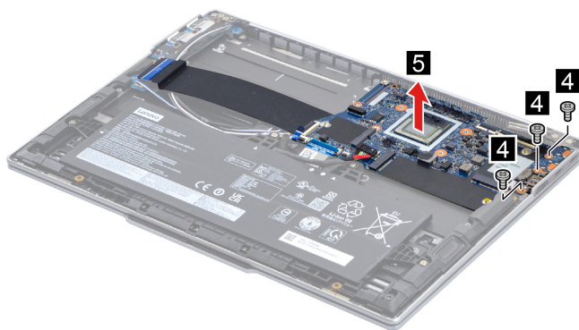
Figure 24. Remove the system board
