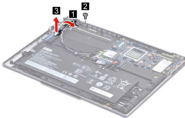
Figure 21. Remove the fingerprint board
