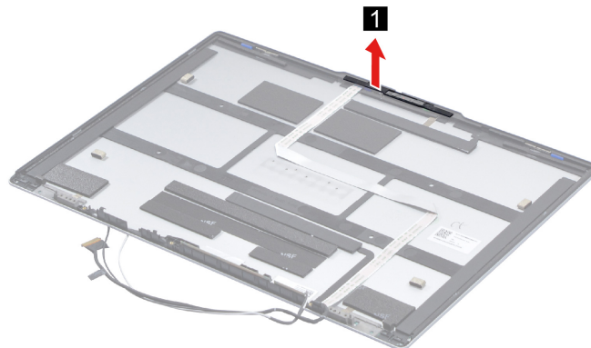
Figure 35. Remove the camera holder
