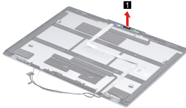
Figure 37. Remove the camera privacy shutter
