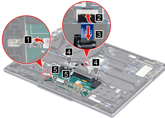
Figure 10. Peel off the tape, disconnect the touchpad cable, and remove four screws
