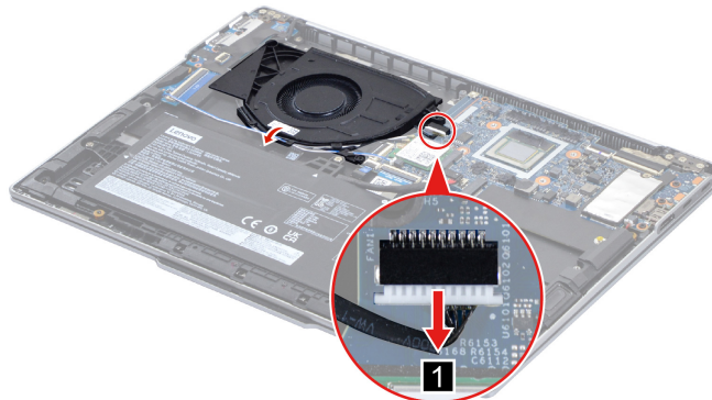
Figure 16. Disconnect the fan cable and release the cable
