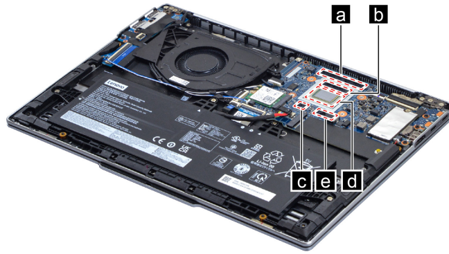
Figure 15. Areas on the system board where thermal interface materials are applied
