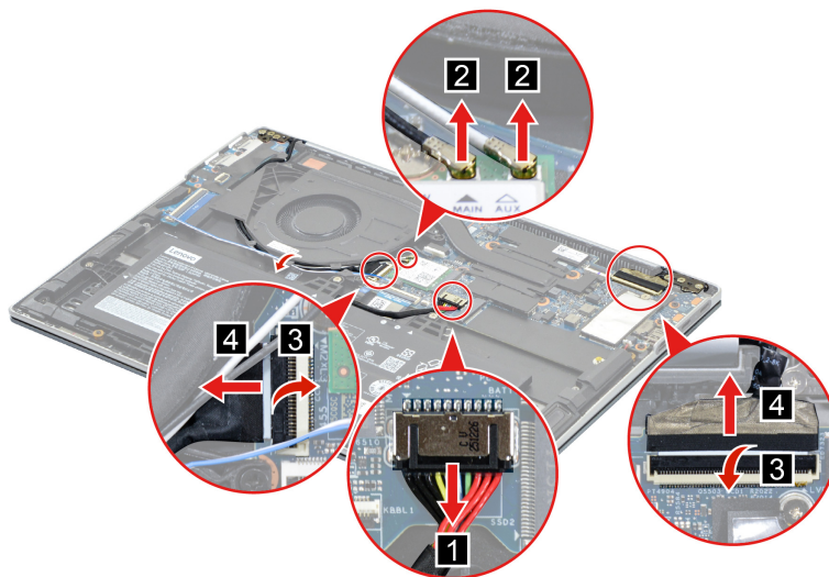
Figure 26. Detach the main and auxiliary antenna cable connectors and disconnect the EDP cable and camera cable
