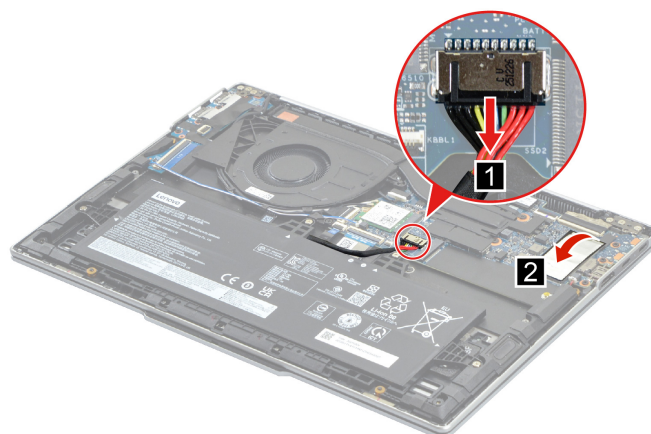
Figure 5. Disconnect the battery pack cable and remove the AL foil mylar
