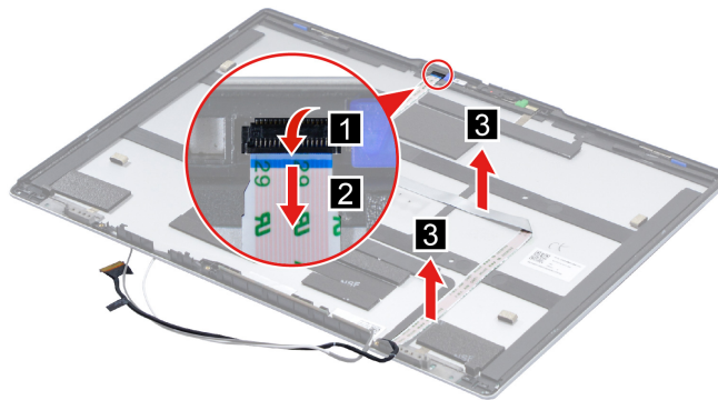
Figure 39. Remove the camera cable
