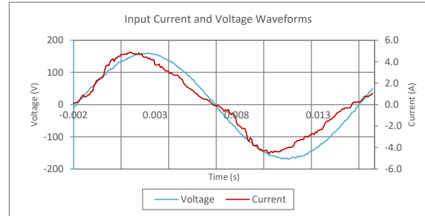
Input AC Current Waveform (THD = 15.37%, 50% Load)
