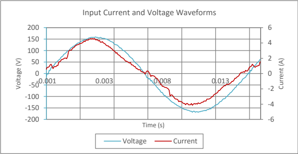
Input AC Current Waveform (ITHD = 13.36%, 50% Load)
