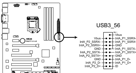
P8Z77-V LE USB3.0 Front panel connector
