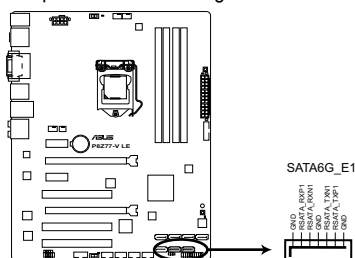
P8Z77-V LE Marvell® SATA 6.0 Gb/s connectors
