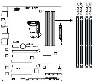
P8Z77-V LE 240-pin DDR3 DIMM sockets
