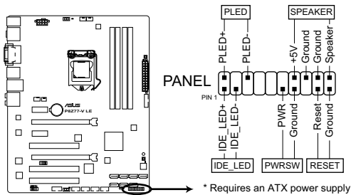
P8Z77-V LE System panel connector
