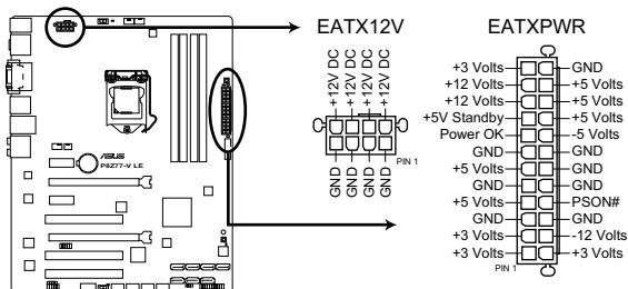
P8Z77-V LE EATX power connectors
