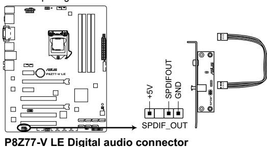
P8Z77-V LE Digital audio connector
