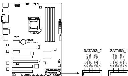
P8Z77-V LE SATA 6.0Gb/s connectors
