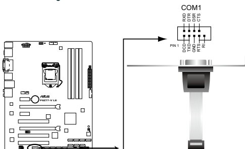
P8Z77-V LE Serial port (COM1) connector
