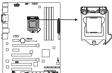
P8Z77-V LE CPU socket LGA1155
