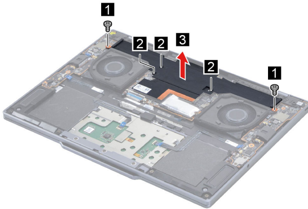
Figure 15. Remove the heat sink
