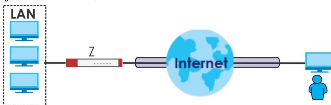
Figure 322 L2TP VPN Overview
