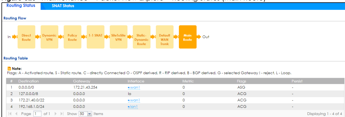
Figure 610 Maintenance > Packet Flow Explore > Routing Status (Main Route)
