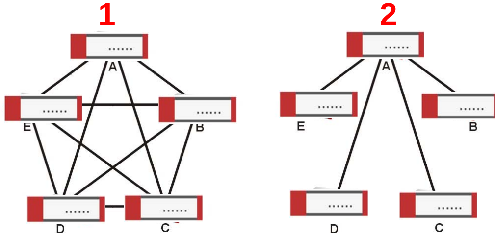
Figure 307 VPN Topologies (Fully Meshed and Hub and Spoke)
