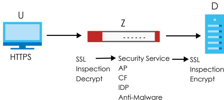
Figure 412 SSL Inspection Overview
