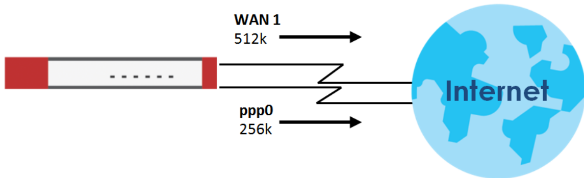
Figure 223 Load Balancing Least Load First Example
