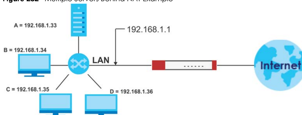
Figure 252 Multiple Servers Behind NAT Example
