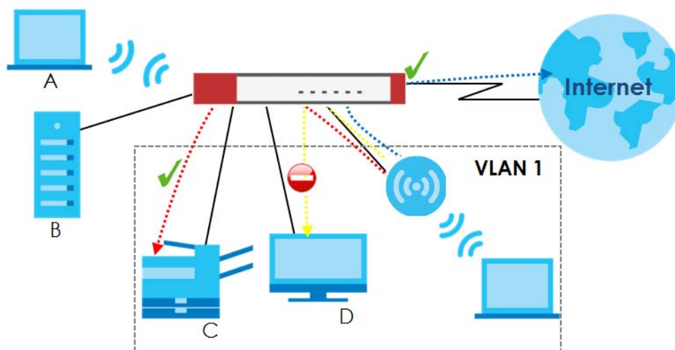
Figure 291 Layer-2 Isolation Application
