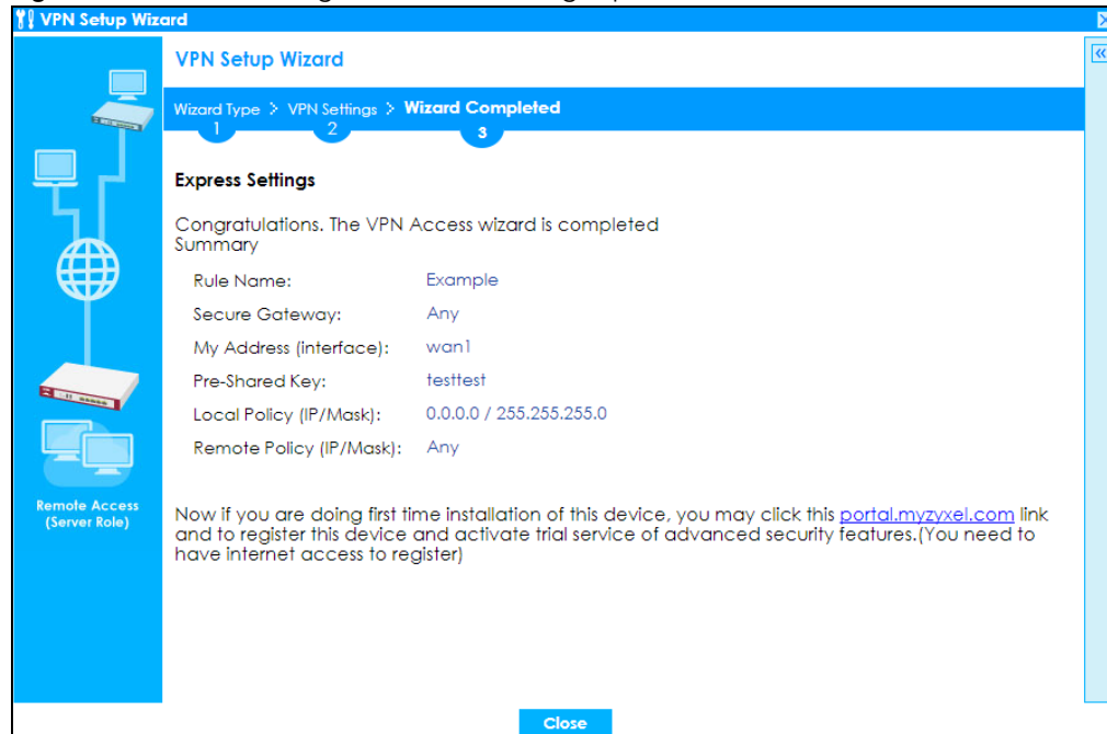
Figure 83 VPN for Configuration Provisioning Express Wizard: Finish
