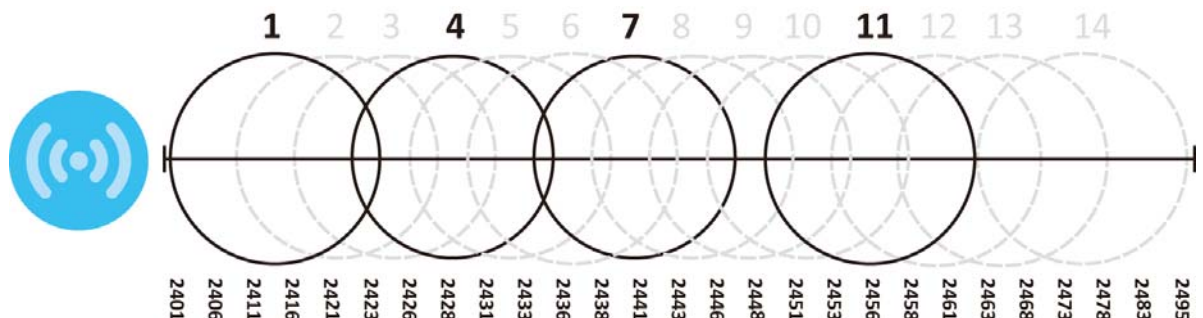
Figure 188 An Example Four-Channel Deployment
