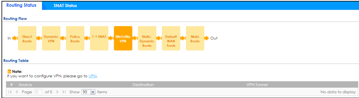
Figure 608 Maintenance > Packet Flow Explore > Routing Status (Static-Dynamic Route)
