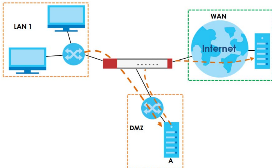
Figure 258 HTTP Redirect Example
