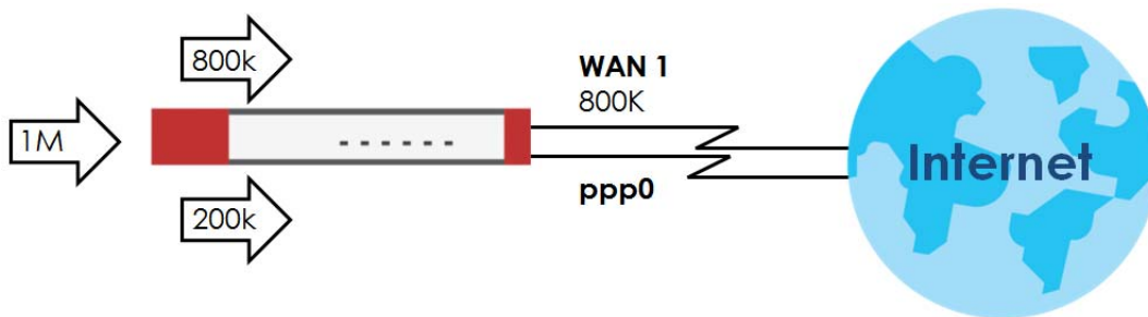
Figure 225 Spillover Algorithm Example
