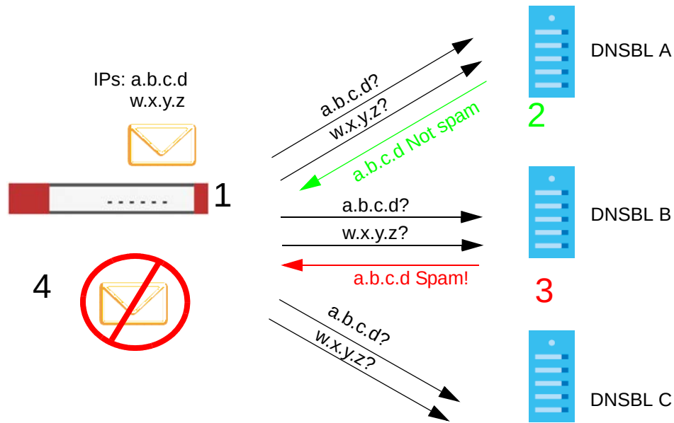
Figure 411 Conflicting DNSBL Replies Example
