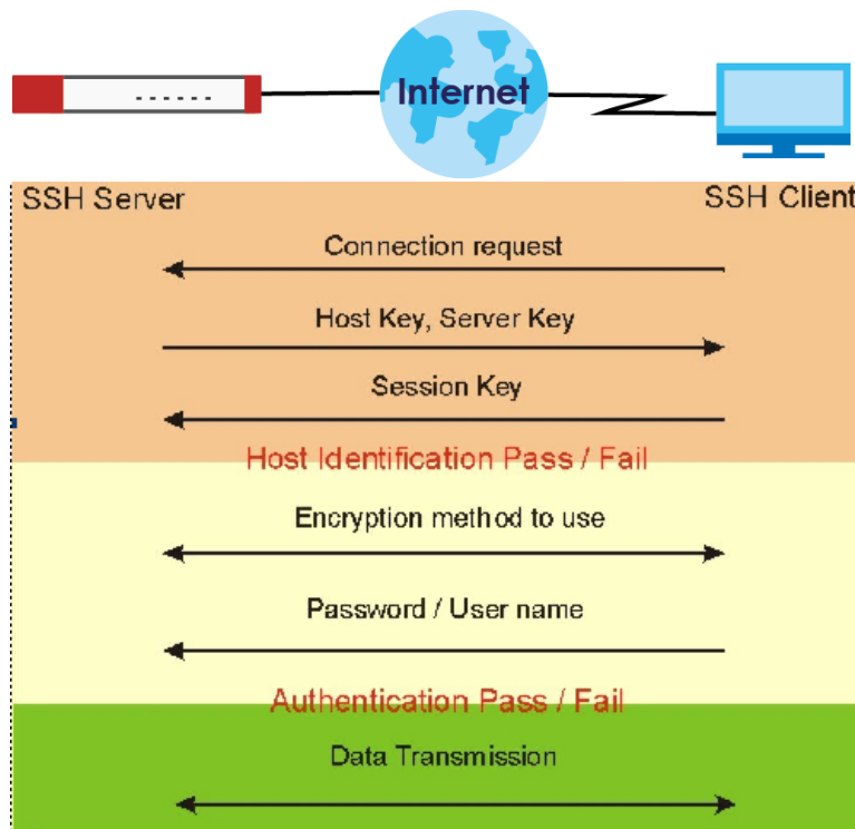
Figure 543 How SSH v1 Works Example
