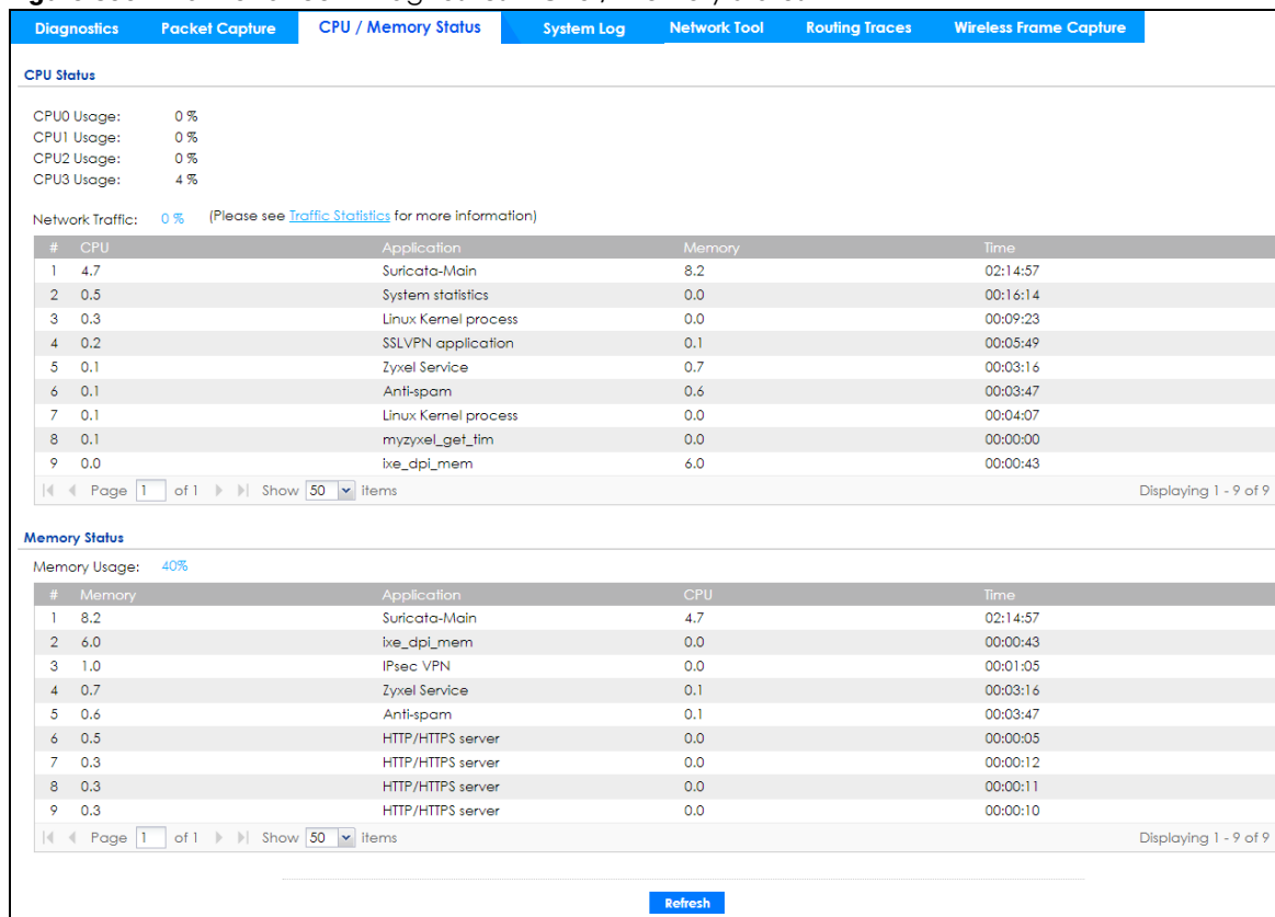
Figure 596 Maintenance > Diagnostics > CPU / Memory Status
