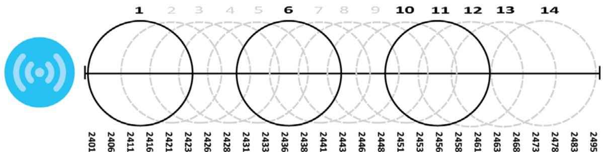
Figure 187 An Example Three-Channel Deployment
