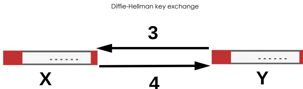
Figure 312 IKE SA: Main Negotiation Mode, Steps 3 - 4: DH Key Exchange
