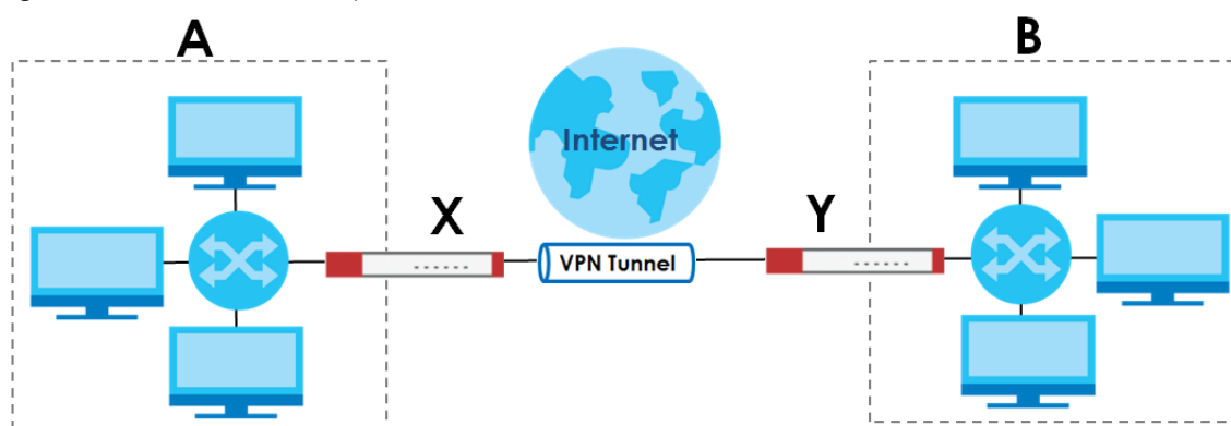
Figure 299 IPSec VPN Example
