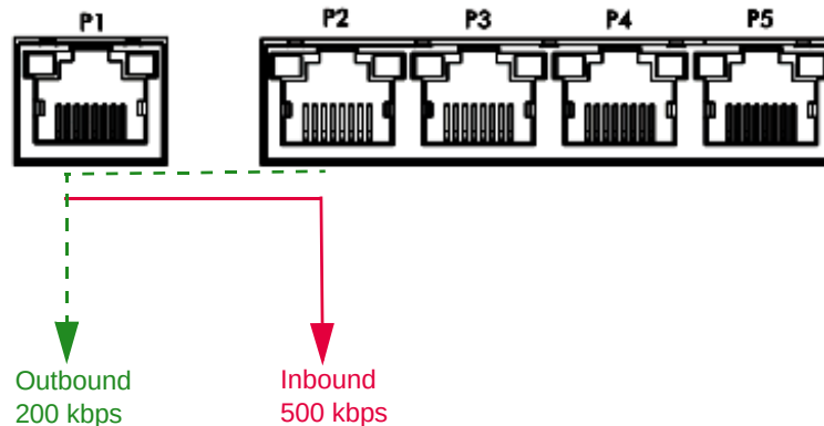
Figure 328 LAN1 to WAN, Outbound 200 kbps, Inbound 500 kbps
