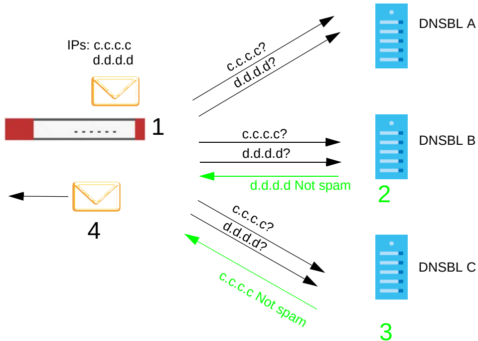
Figure 410 DNSBL Legitimate Email Detection Example
