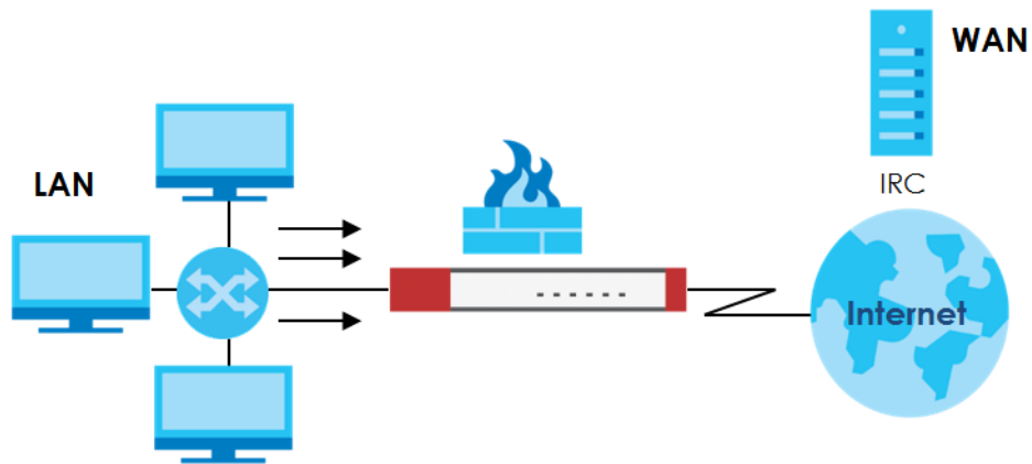
Figure 369 Blocking All LAN to WAN IRC Traffic Example
