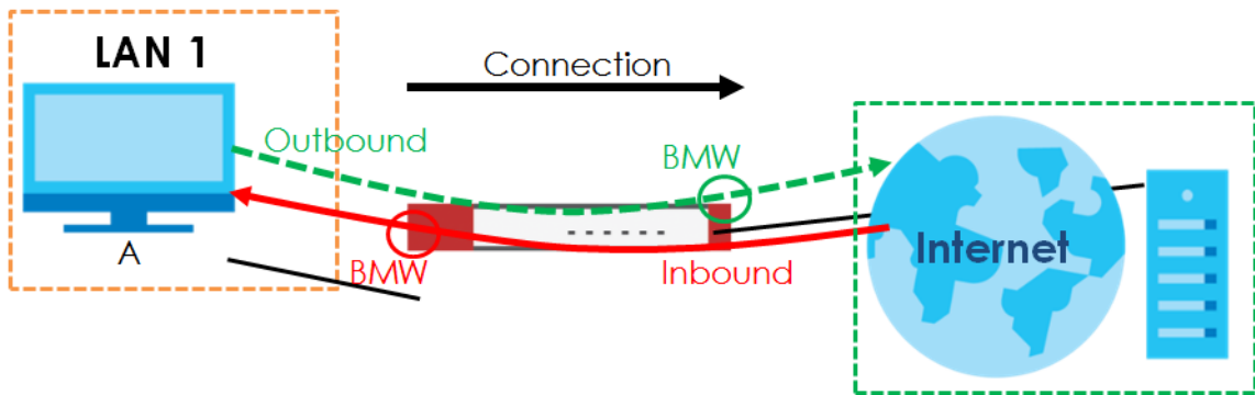
Figure 327 LAN1 to WAN Connection and Packet Directions
