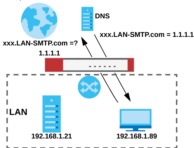
Figure 255 LAN Computer Queries a Public DNS Server
