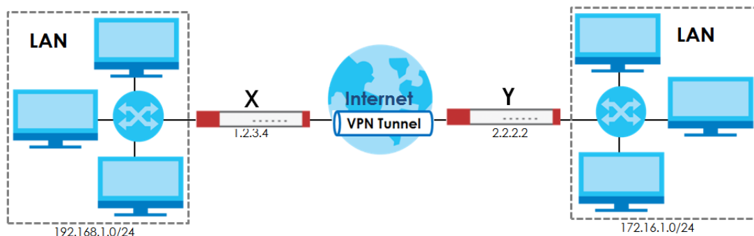
Figure 317 Site-to-site IPSec VPN Example
