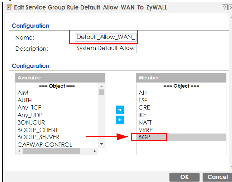
Figure 245 Allow BGP to the Zyxel Device
