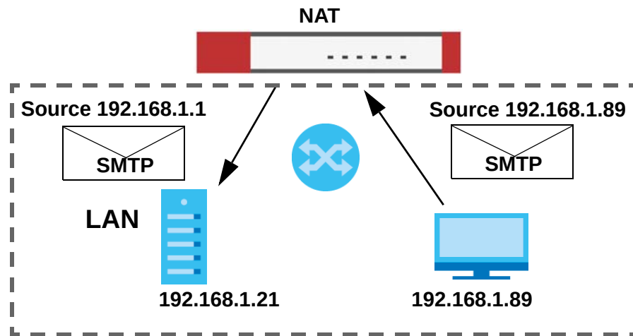
Figure 256 LAN to LAN Traffic
