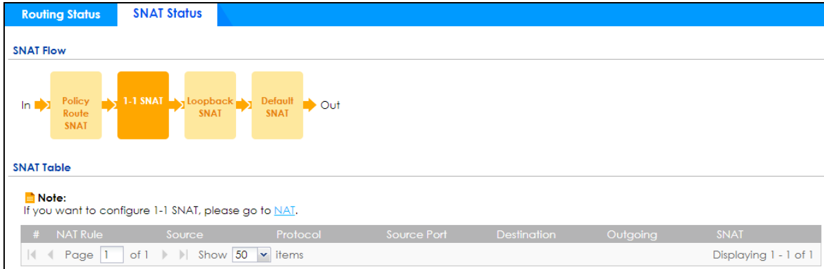
Figure 613 Maintenance > Packet Flow Explore > SNAT Status (Loopback SNAT)
