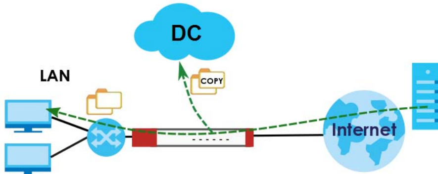
Figure 403 General Zyxel Sandbox Inspection
