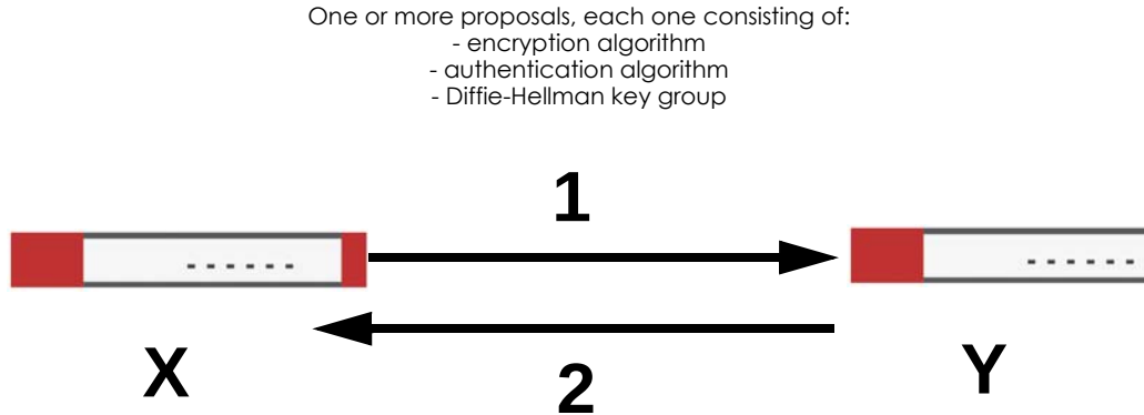
Figure 311 IKE SA: Main Negotiation Mode, Steps 1 - 2: IKE SA Proposal
