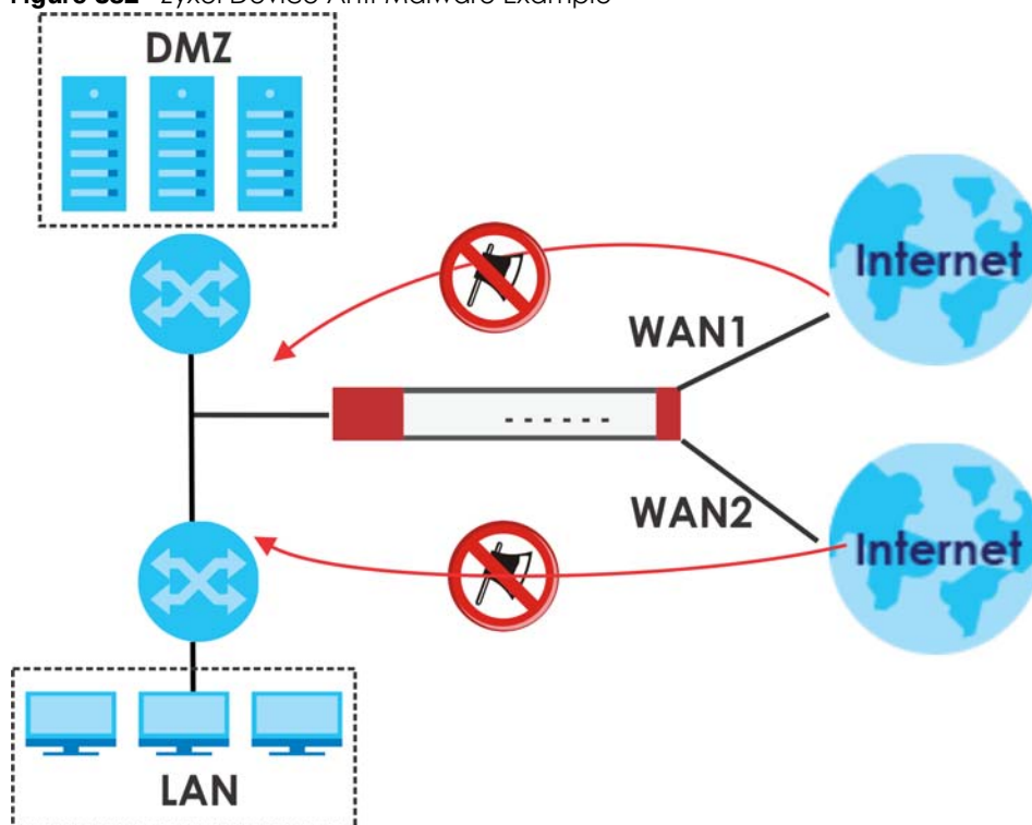
Figure 382 Zyxel Device Anti-Malware Example
