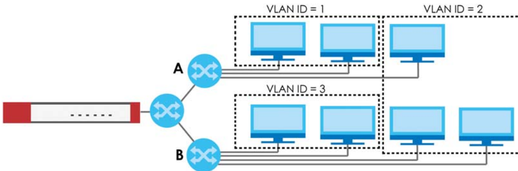
Figure 215 Example: After VLAN
