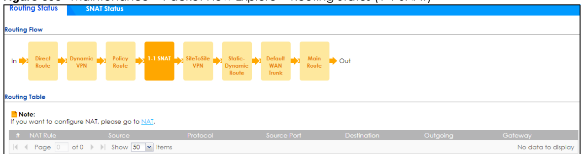
Figure 606 Maintenance > Packet Flow Explore > Routing Status (1-1 SNAT)
