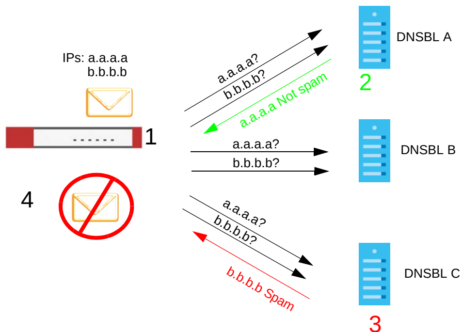
Figure 409 DNSBL Spam Detection Example
