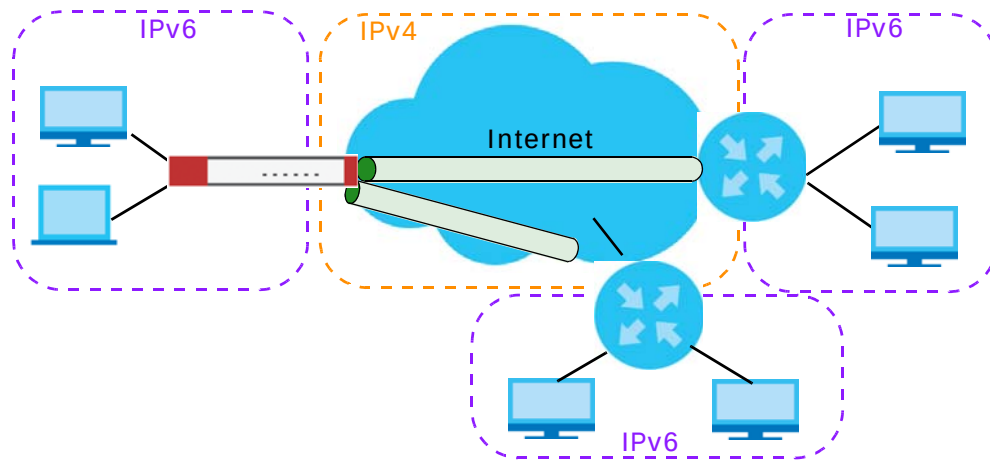
Figure 211 6to4 Tunnel
