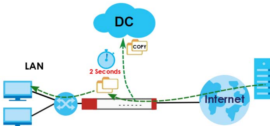
Figure 404 Advanced Zyxel Sandbox Inspection
