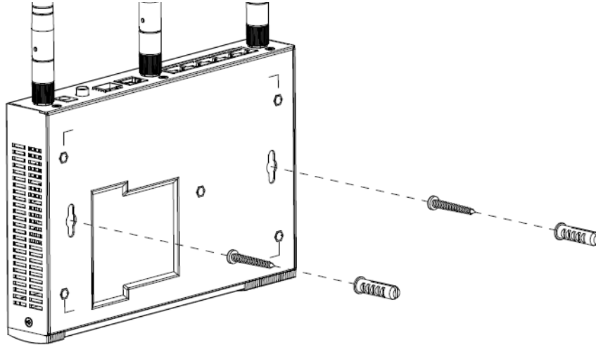
Figure 56 Wall Mounting
