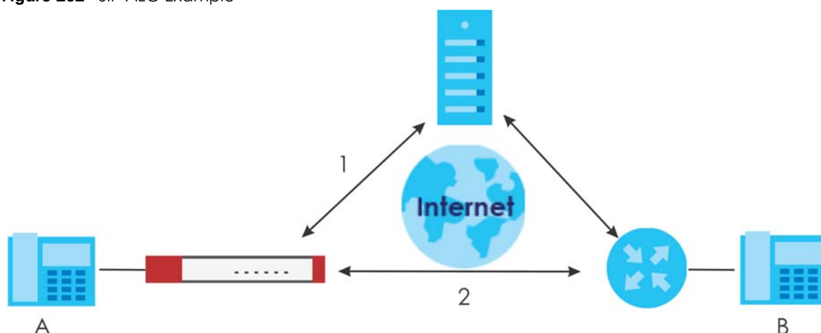
Figure 262 SIP ALG Example
