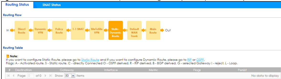
Figure 609 Maintenance > Packet Flow Explore > Routing Status (Default WAN Trunk)
