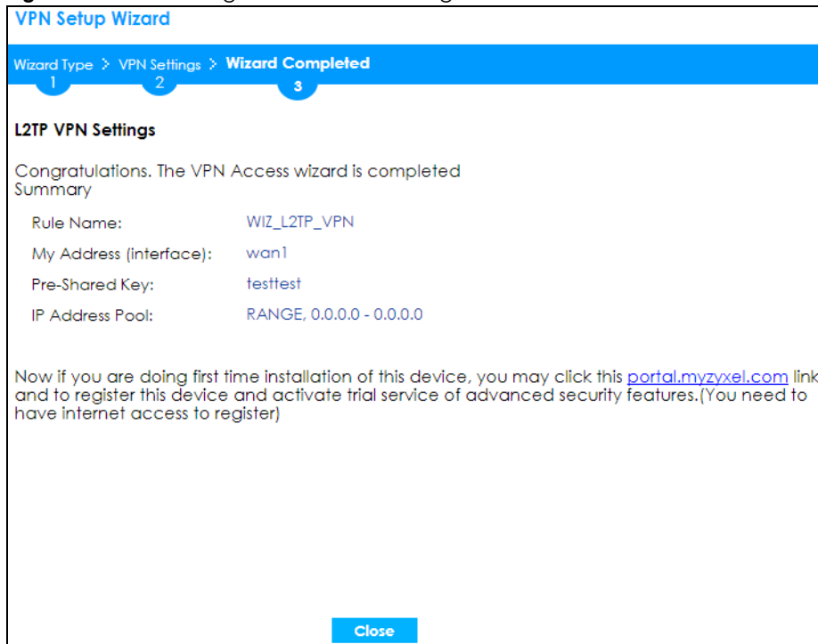
Figure 93 VPN Settings for L2TP VPN Settings Wizard: Finish
