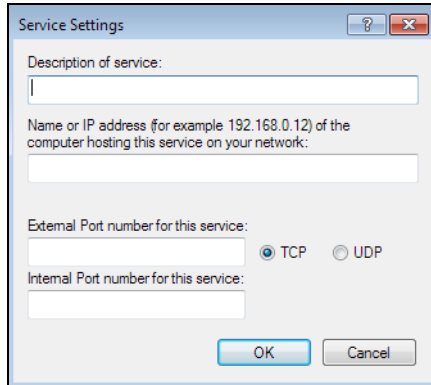
Figure 271 Internet Connection Properties: Advanced Settings: Add
