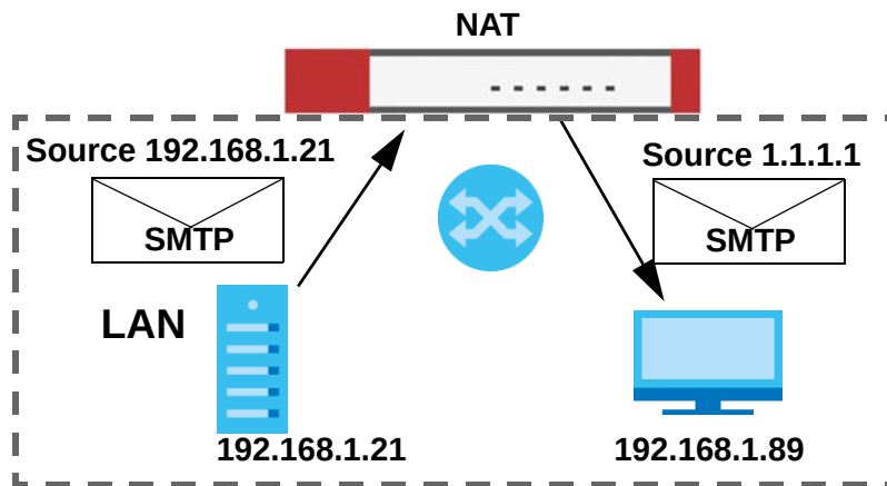
Figure 257 LAN to LAN Return Traffic
