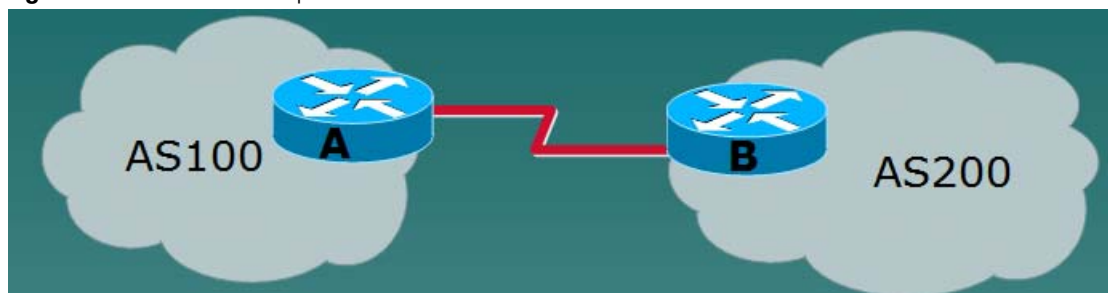
Figure 244 eBGP Concept
