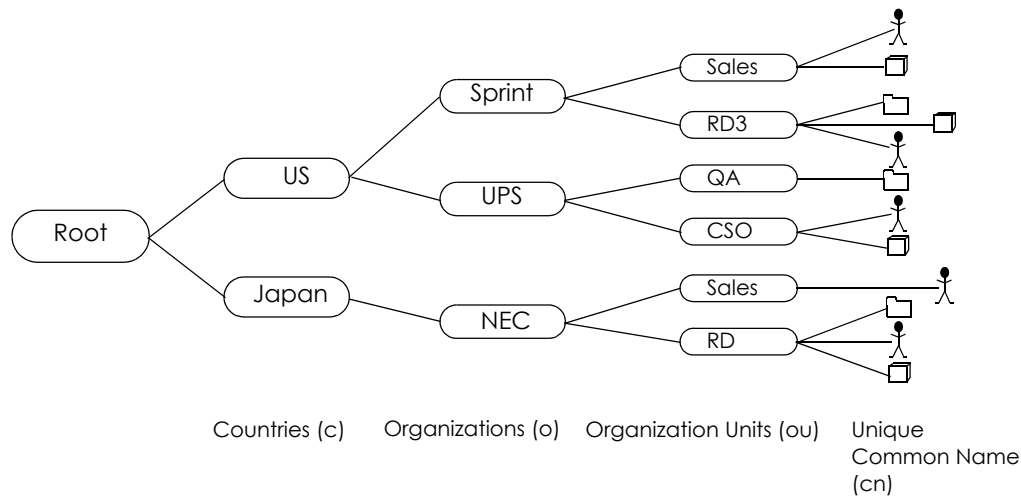
Figure 468 Basic Directory Structure
