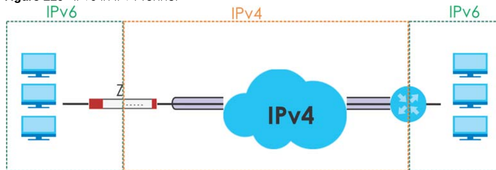
Figure 210 IPv6-in-IPv4 Tunnel
