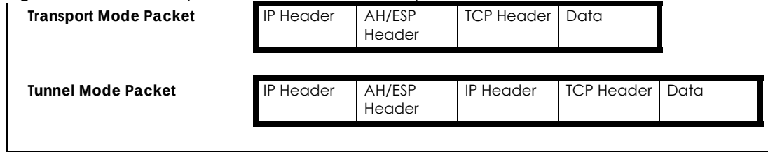
Figure 315 VPN: Transport and Tunnel Mode Encapsulation
