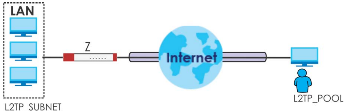
Figure 323 Policy Route for L2TP VPN
