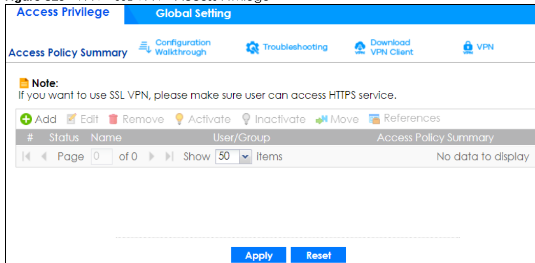
Figure 319 VPN > SSL VPN > Access Privilege
