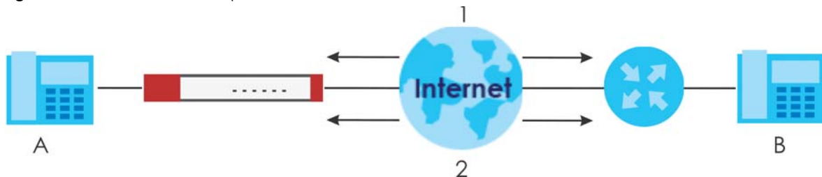
Figure 263 H.323 ALG Example
