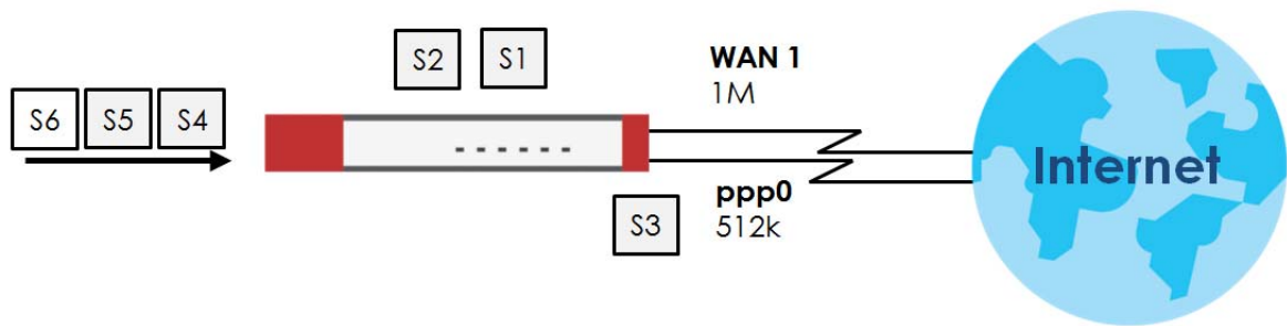
Figure 224 Weighted Round Robin Algorithm Example
