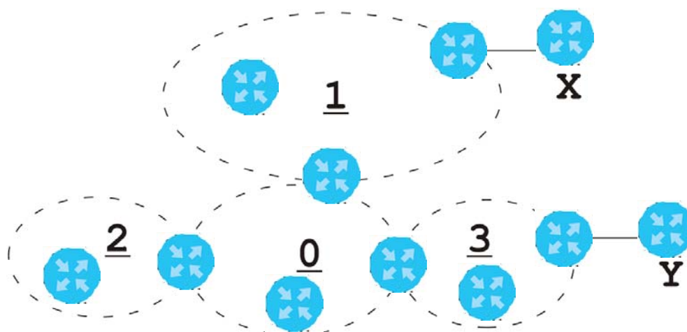
Figure 238 OSPF: Types of Areas
