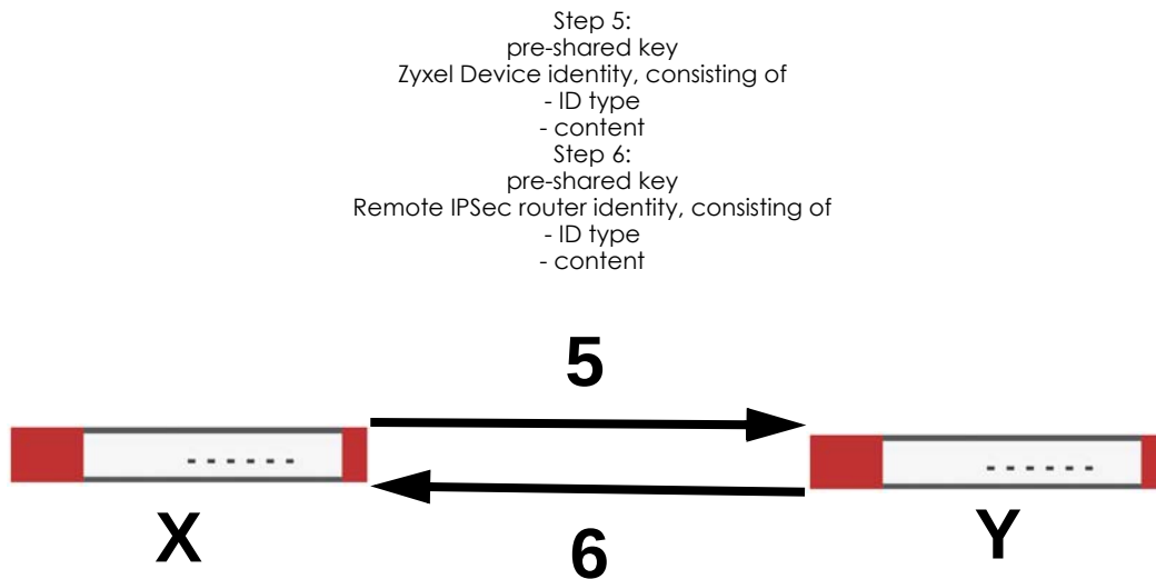
Figure 313 IKE SA: Main Negotiation Mode, Steps 5 - 6: Authentication (continued)
