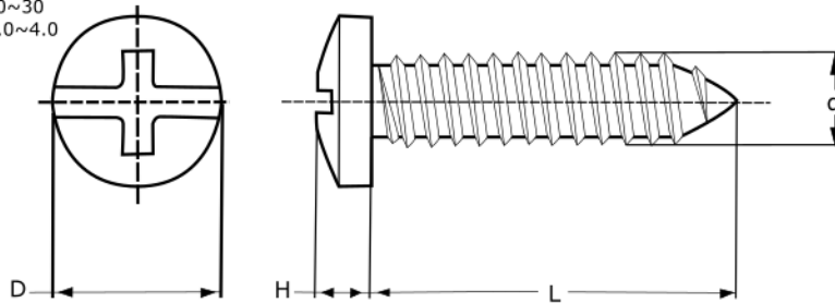
Figure 55 Wall mounting screw specifications
