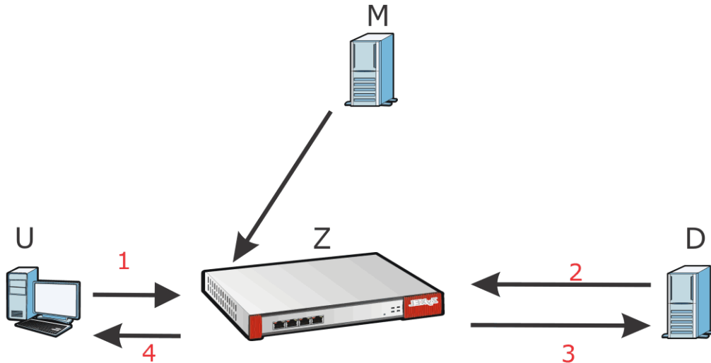
Figure 417 SSL Inspection Certificate Update Overview
