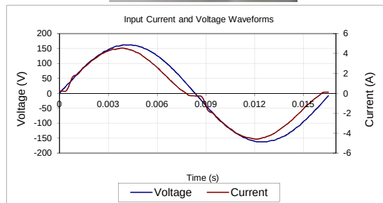
Input AC Current Waveform (ITHD = 10.87%, 50% Load)
