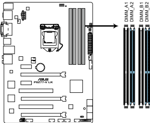
P8Z77-V LK 240-pin DDR3 DIMM sockets
