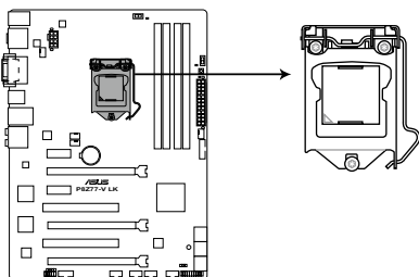
P8Z77-V LK CPU socket LGA1155
