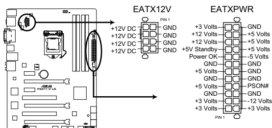
P8Z77-V LK ATX power connectors
