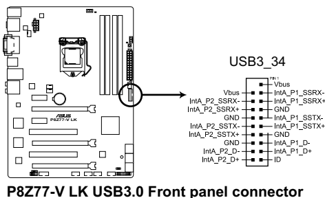
P8Z77-V LK USB3.0 Front panel connector
