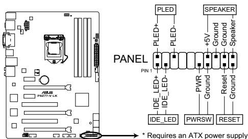
P8Z77-V LK System panel connector
