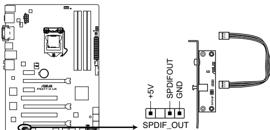
P8Z77-V LK Digital audio connector
