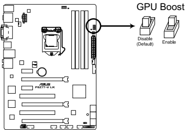
P8Z77-V LK GPU Boost switch
