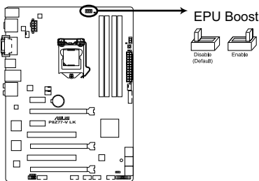
P8Z77-V LK EPU Boost switch
