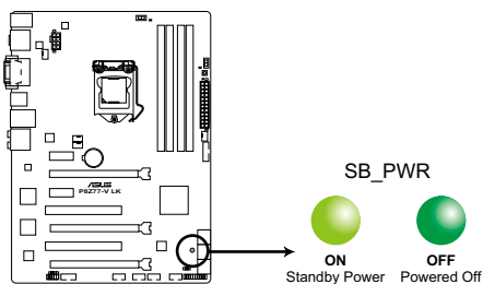
P8Z77-V LK Onboard LED
