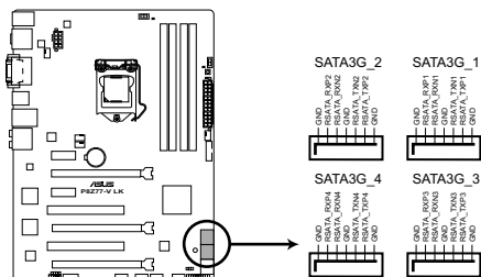
P8Z77-V LK SATA 3.0Gb/s connectors
