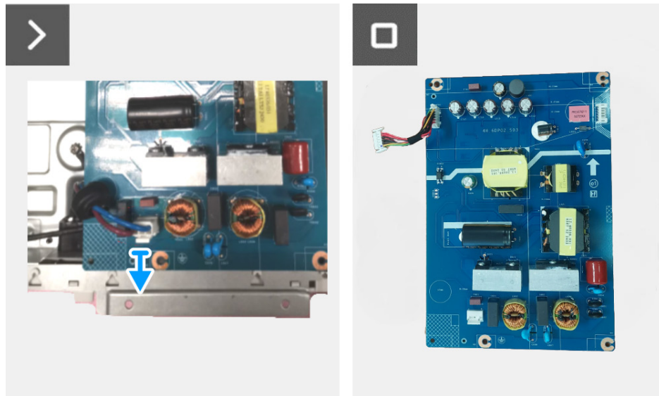
Figure 15. Removing the power board
