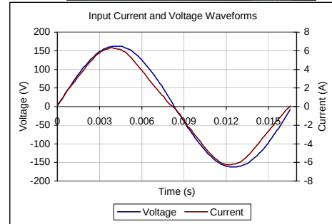
Input AC Current Waveform (THD = 7.51%, 50% Load)
