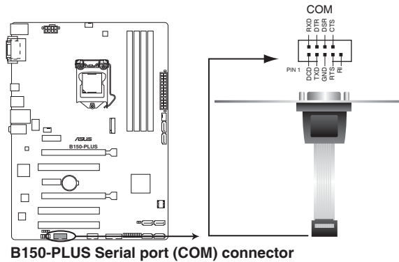
B150-PLUS Serial port (COM) connector
