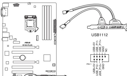
B150-PLUS USB2.0 connector
