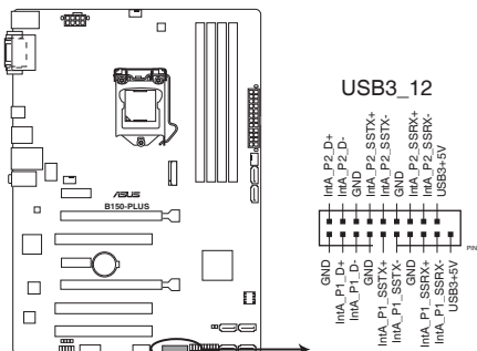
B150-PLUS USB3.0 Front panel connector
