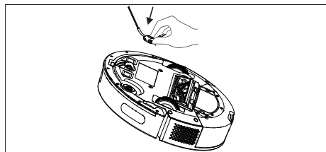
Fig. 10 – Inserting the side brush
