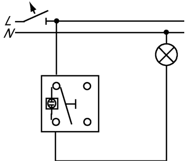
1gang 1way SP
