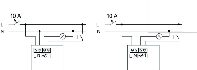
Wiring diagram
