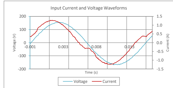
Input AC Current Waveform (ITHD = 11.11%, 50% Load)
