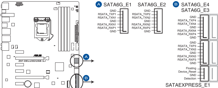
Z97-DELUXE/USB 3.1 ASMedia® SATA 6 Gb/s connectors
