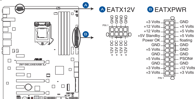
Z97-DELUXE/USB 3.1 ATX power connectors
