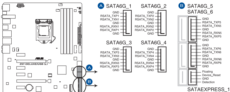
Z97-DELUXE/USB 3.1 Intel® SATA 6 Gb/s connectors
