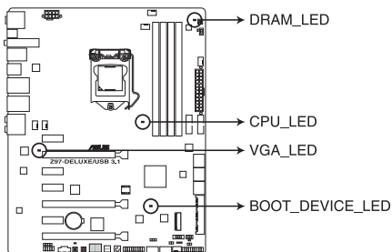
Z97-DELUXE/USB 3.1 CPU/ DRAM/ BOOT_DEVICE/ VGA LED
