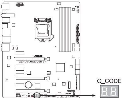
Z97-DELUXE/USB 3.1 Q-Code LED
