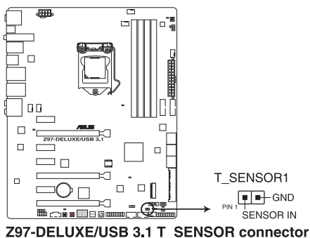
Z97-DELUXE/USB 3.1 T_SENSOR connector
