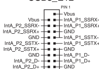
Z97-DELUXE/USB 3.1 USB3.0 connectors
