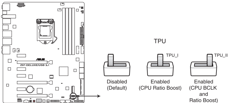
Z97-DELUXE/USB 3.1 TPU switch
