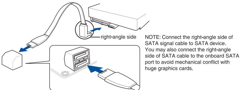
Z97-DELUXE/USB 3.1 Intel® SATA 6 Gb/s connectors
