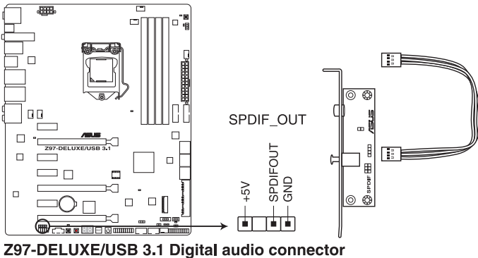
Z97-DELUXE/USB 3.1 Digital audio connector
