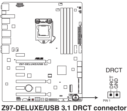
Z97-DELUXE/USB 3.1 DRCT connector
