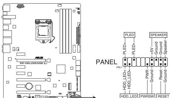
Z97-DELUXE/USB 3.1 System panel connector
