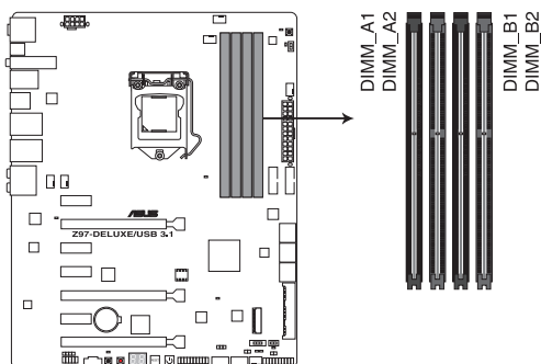
Z97-DELUXE/USB 3.1 240-pin DDR3 DIMM socket
