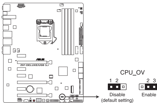
Z97-DELUXE/USB 3.1 CPU_OV setting
