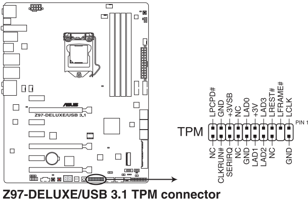
Z97-DELUXE/USB 3.1 TPM connector
