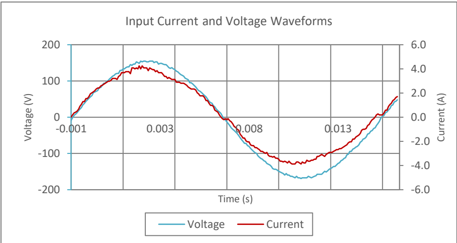
Input AC Current Waveform (ITHD = 4.39%, 50% Load)
