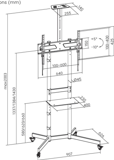
Dimensions (mm)
