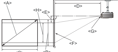
Deckeninstallation
