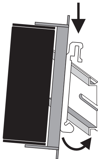
Figure 6: Assembly on carrier rail 1
