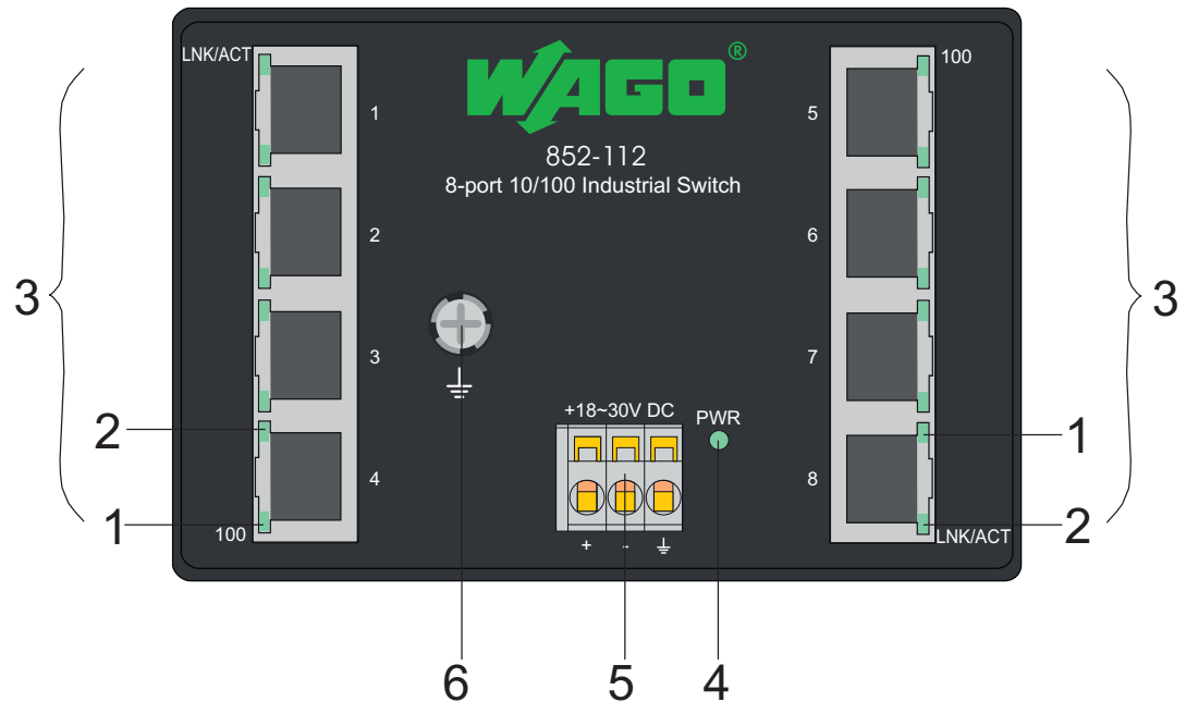
Figure 1: Front view of Industrial Eco Switch
