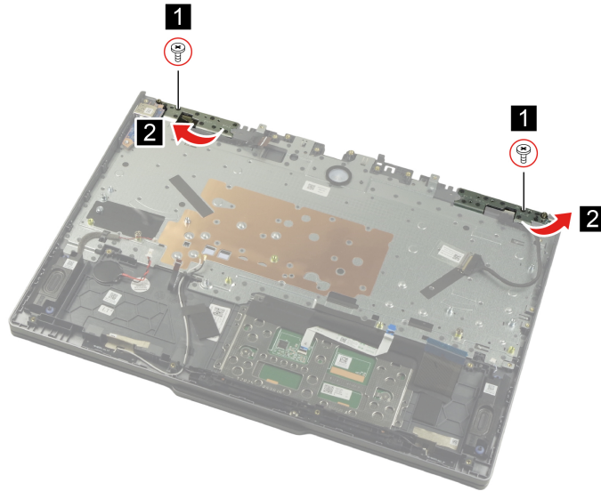
Figure 34. Remove two screws and peel off the cables
