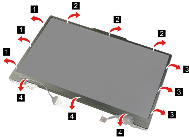
Figure 36. Remove the LCD bezel
