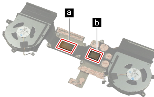
Figure 25. LOQ 15IPH11–Areas on the heat sink where thermal interface materials should be applied
