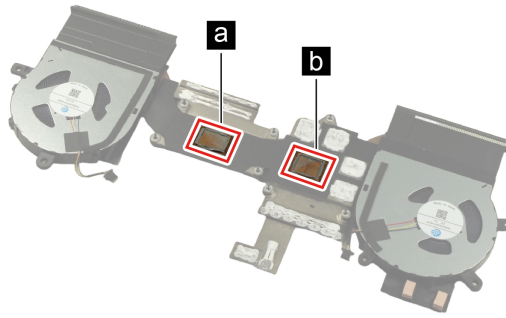
Figure 24. LOQ 15AHP11–Areas on the heat sink where thermal interface materials should be applied
