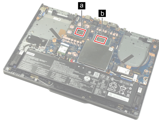
Figure 27. LOQ 15IPH11—Areas on the system board where thermal interface materials are applied
