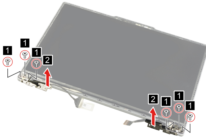
Figure 38. Remove the hinges
