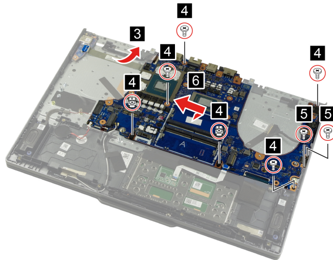
Figure 30. Remove the system board
