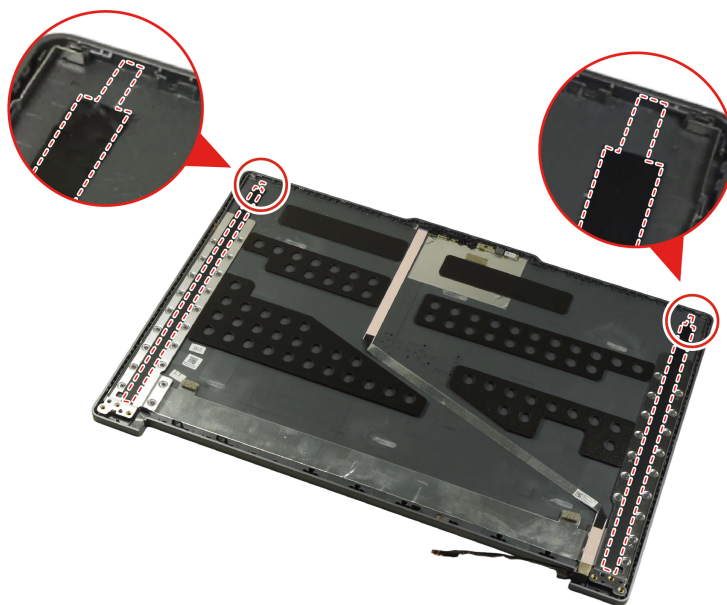
Figure 41. The locations of the stretch-release tapes
