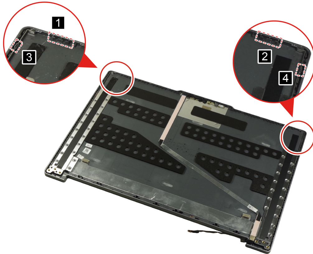
Figure 42. The locations where the rubber pads should be adhered
