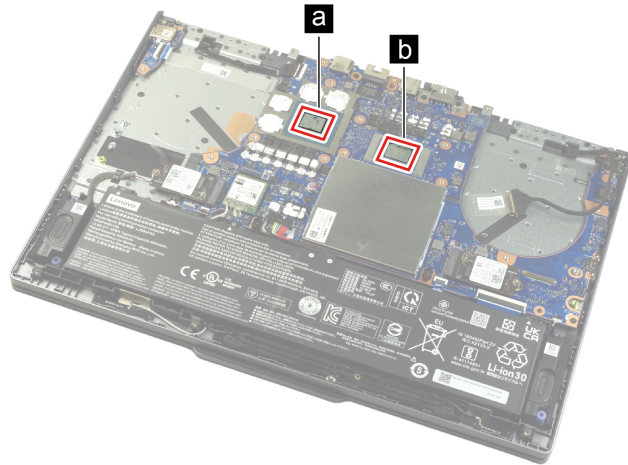
Figure 26. LOQ 15AHP11—Areas on the system board where thermal interface materials are applied
