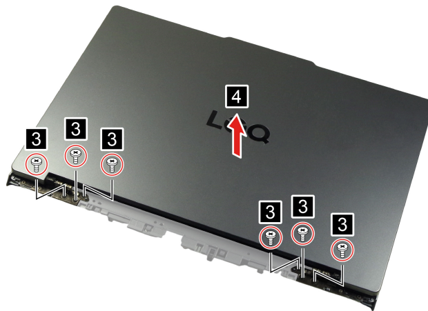
Figure 35. Remove six screws and remove the LCD module
