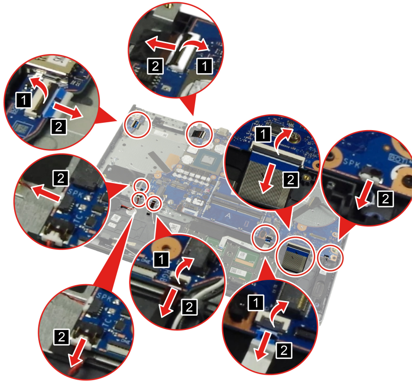
Figure 29. Disconnect the cables connected to the system board
