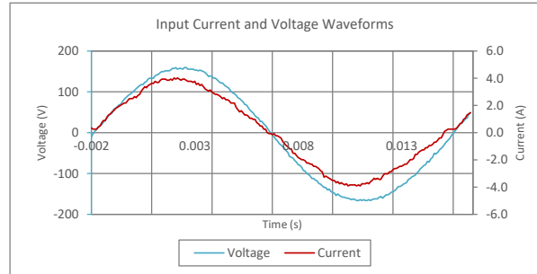
Input AC Current Waveform (ITHD = 6.11%, 50% Load)
