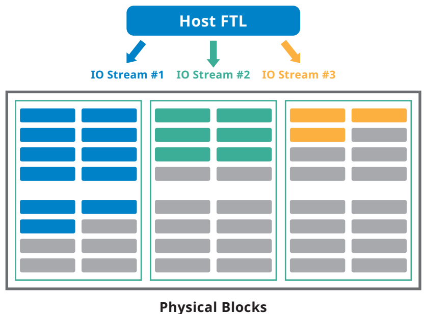
Fig. 2: when FTL is implemented on the host side, the host can maintain appropriate I/O isolation and optimize data placement
