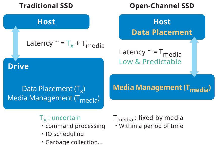
Fig. 2: when FTL is implemented on the host side, the host can maintain appropriate I/O isolation and optimize data placement
