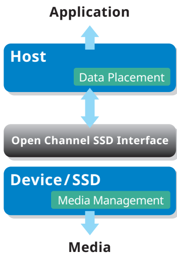
Fig. 1: the Open Channel architecture provides for partitioning of data placement and media management
