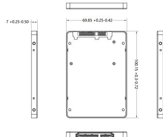
Figure 1-1 Dimensions (mm)
