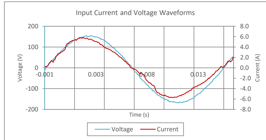
Input AC Current Waveform (ITHD = 8.97%, 50% Load)
