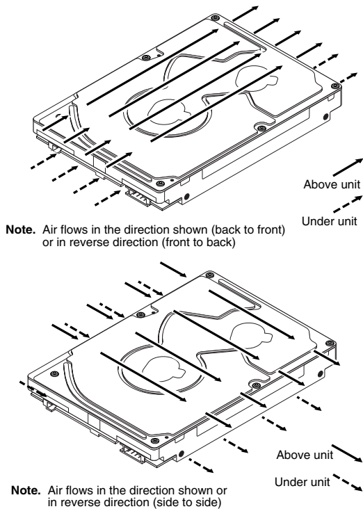
Figure 5. Air flow
