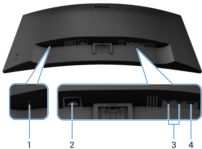
Figure 3. Bottom view
