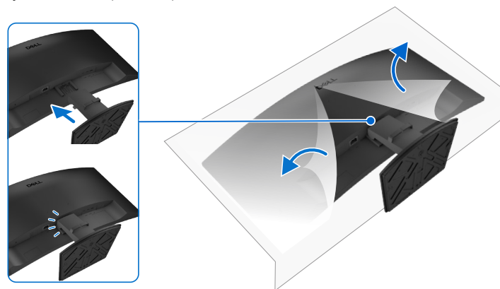
Figure 11. Attach the stand
