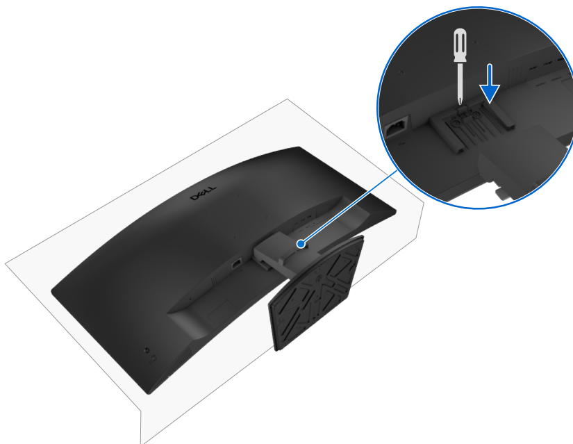
Figure 20. Removing the monitor stand
