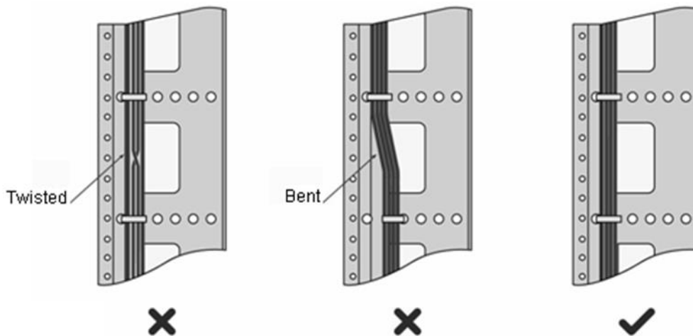
Figure 6-4 Bundling Up Cables (1)
