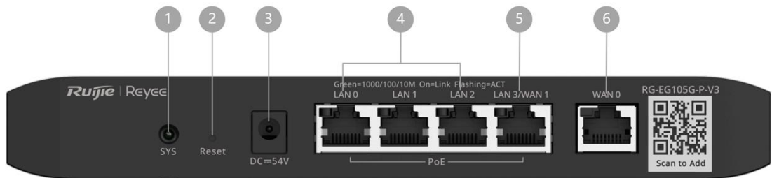
Figure 1-2 Front Panel of RG-EG105G-P-V3
