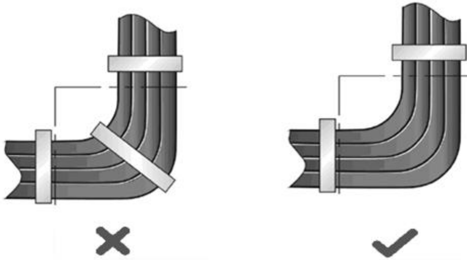
Figure 6-6 Bundling Up Cables (3)
