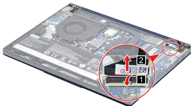
Figure 40. Disconnect the EDP cable from the system board
