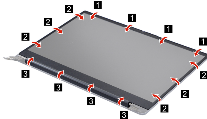
Figure 77. Remove the panel bezel
