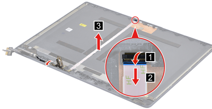
Figure 82. Remove the EDP cable
