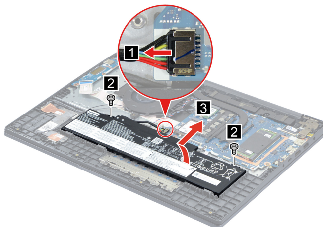
Figure 56. Remove the battery pack
