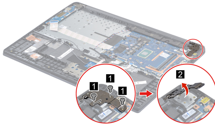
Figure 71. Remove three screws and flip the hinge
