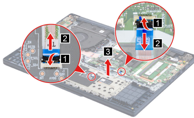
Figure 17. Remove the touchpad cable
