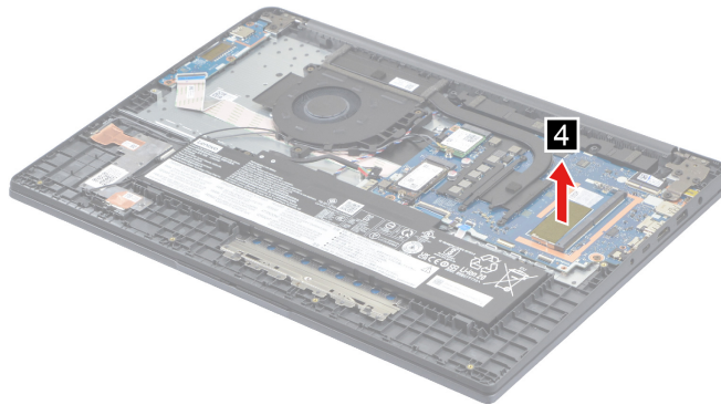
Figure 62. Remove the DDR absorber
