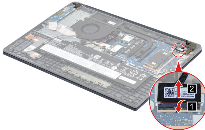
Figure 75. Disconnect the EDP cable from the system board
