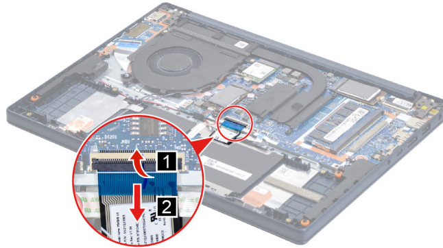
Figure 15. Disconnect the keyboard cable
