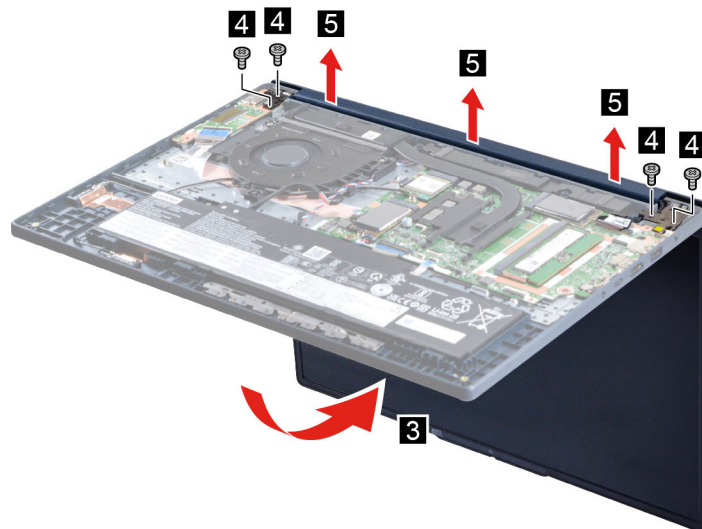
Figure 43. Remove the display assembly (16-inch models)
