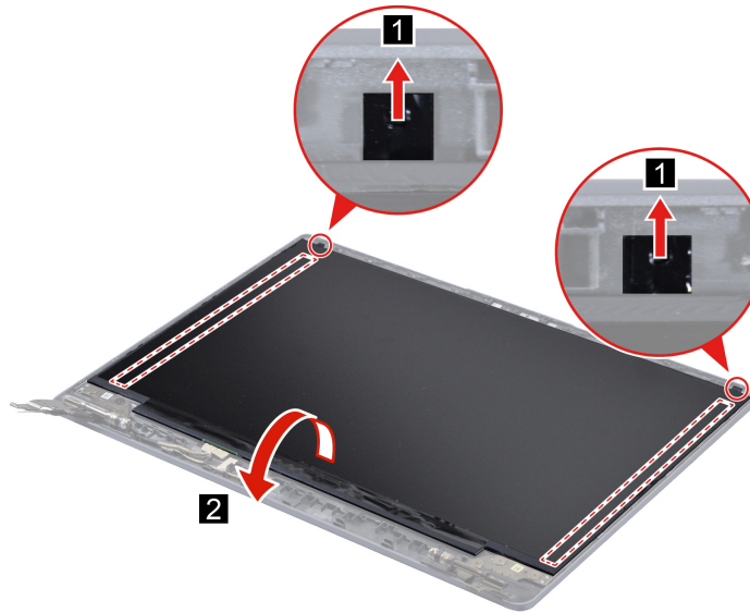
Figure 79. Remove the removable tape and turn over the panel
