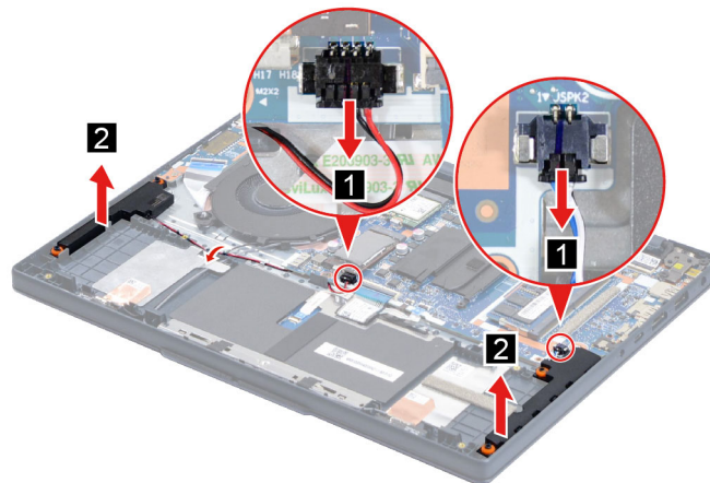
Figure 18. Remove the speaker (14-inch models)
