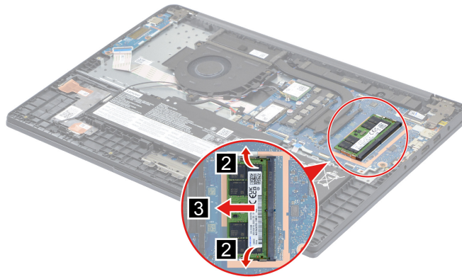
Figure 61. Remove the memory module
