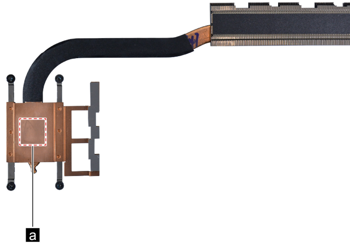
Figure 66. Areas on the heat sink where thermal interface materials should be applied
