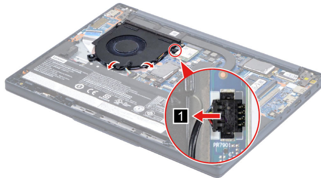
Figure 23. Disconnect the fan cable
