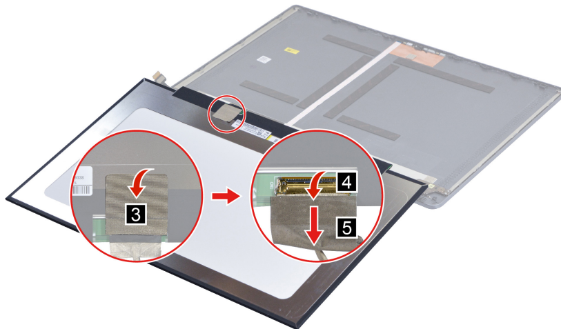
Figure 80. Remove the panel
