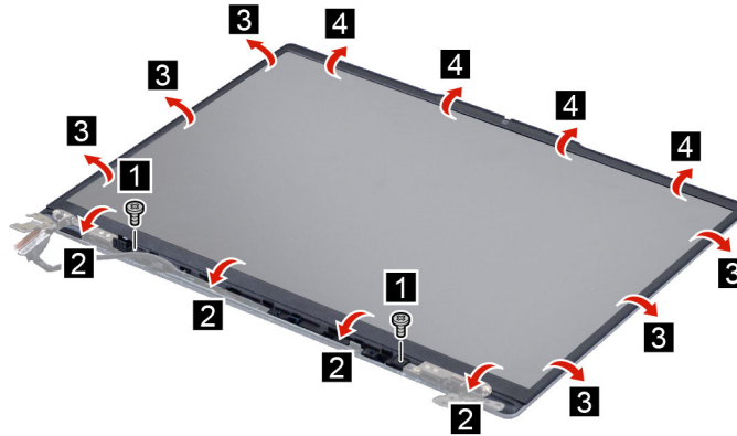
Figure 45. Remove the panel bezel
