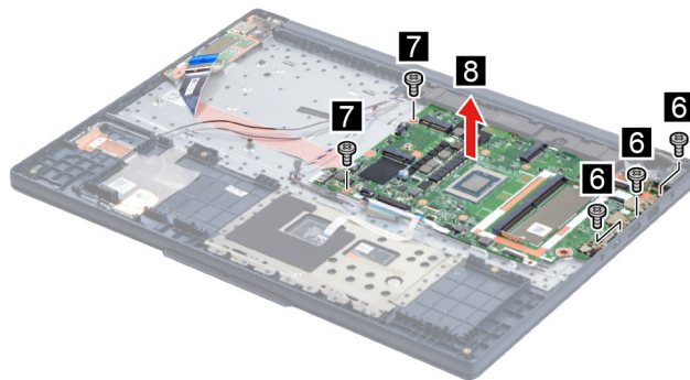
Figure 38. Remove the system board
