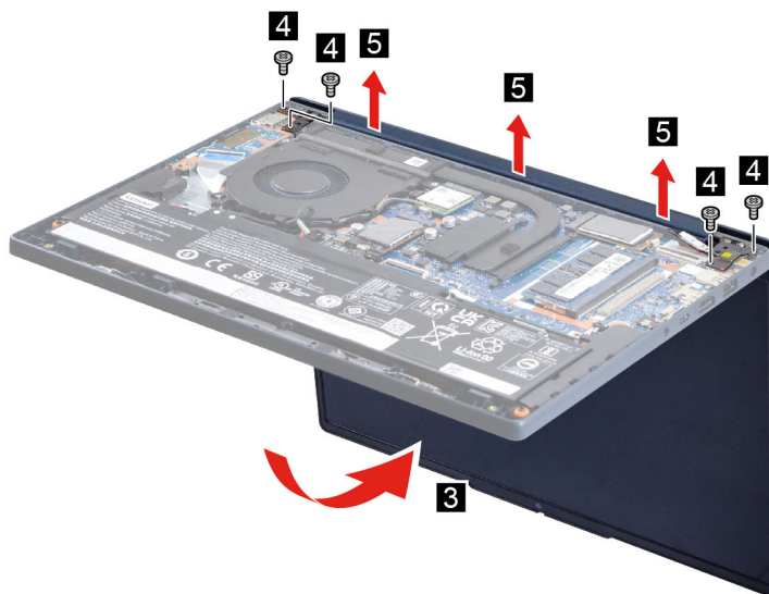
Figure 41. Remove the display assembly (14-inch models)
