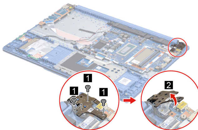
Figure 32. Remove three screws and flip the hinge
