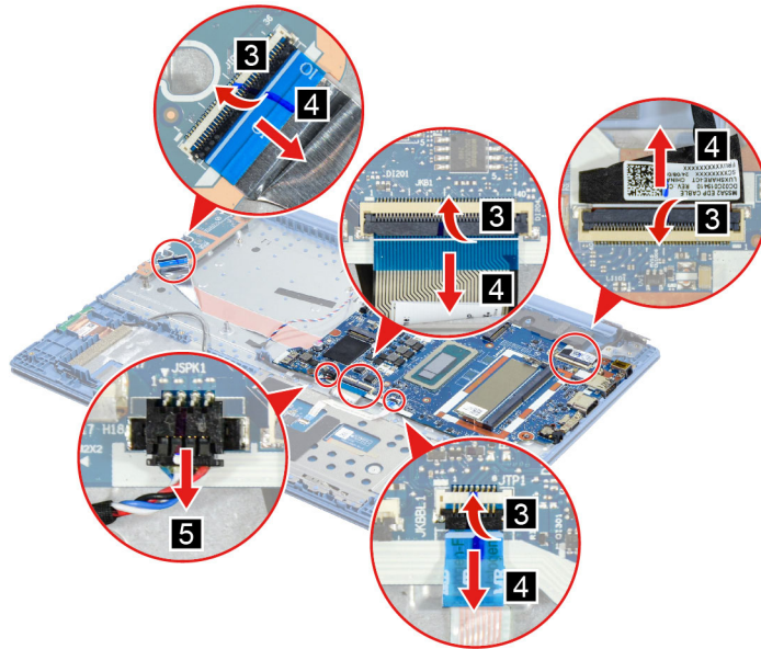
Figure 33. Disconnect cables connected to the system board
