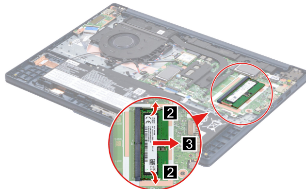
Figure 13. Remove the memory module (16-inch models)
