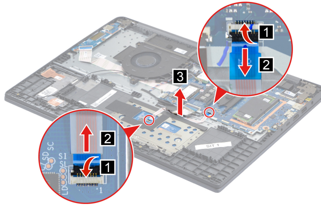
Figure 63. Remove the touchpad cable
