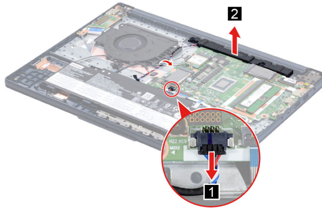
Figure 19. Remove the speaker (15-inch models/16-inch models)
