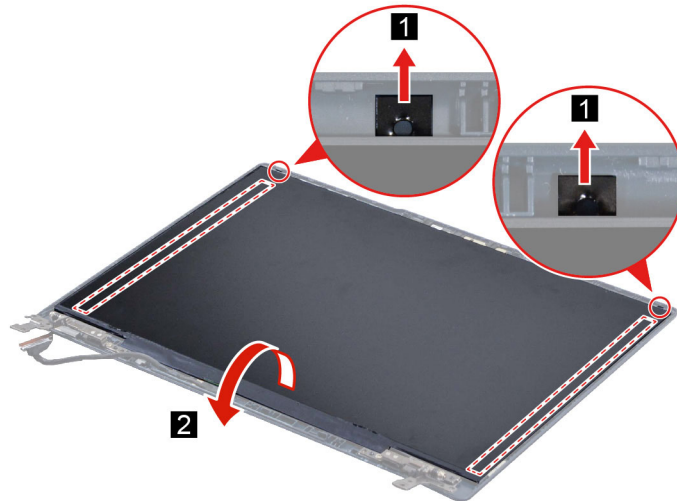
Figure 46. Remove the removable tape and turn over the panel
