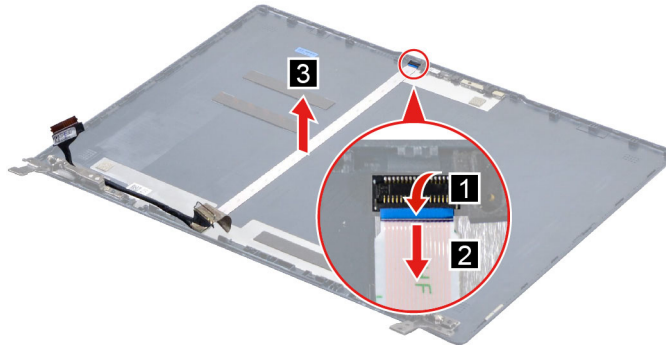
Figure 51. Remove the EDP cable
