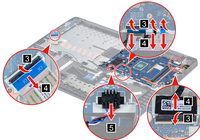
Figure 72. Disconnect the I/O board cable and disconnect cables connected to the system board
