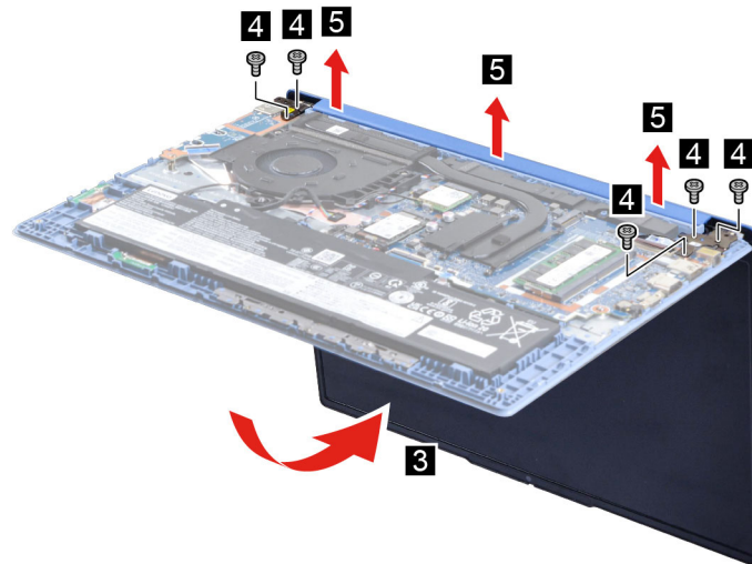
Figure 42. Remove the display assembly (15-inch models)
