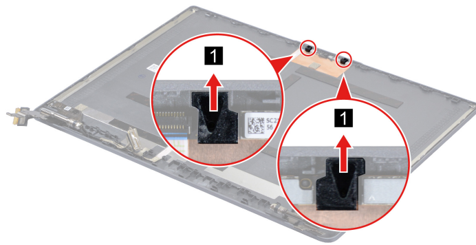
Figure 81. Remove the microphone rubbers
