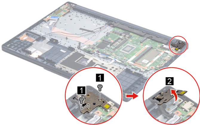
Figure 36. Remove two screws and flip the hinge
