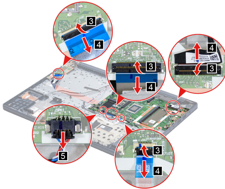
Figure 37. Disconnect cables connected to the system board
