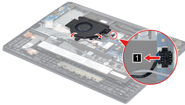
Figure 68. Disconnect the fan cable
