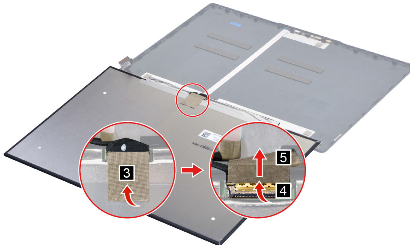
Figure 47. Remove the panel
