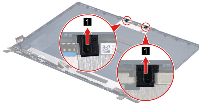
Figure 50. Remove the microphone rubbers
