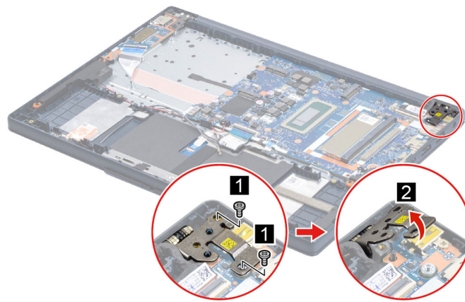
Figure 28. Remove two screws and flip the hinge
