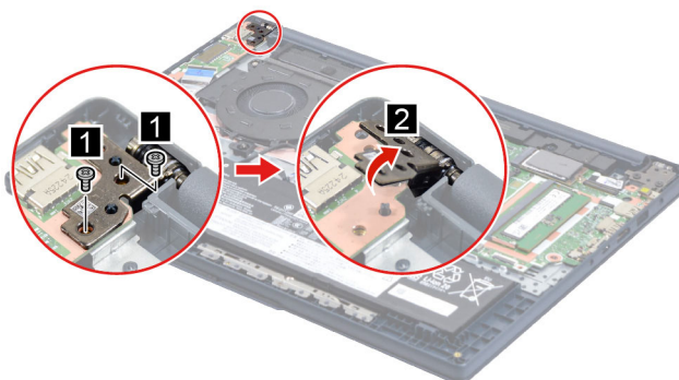
Figure 26. Flip the hinge (15-inch models/16-inch models)
