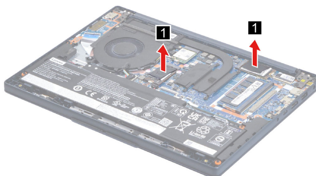
Figure 8. Remove the SSD thermal pad
