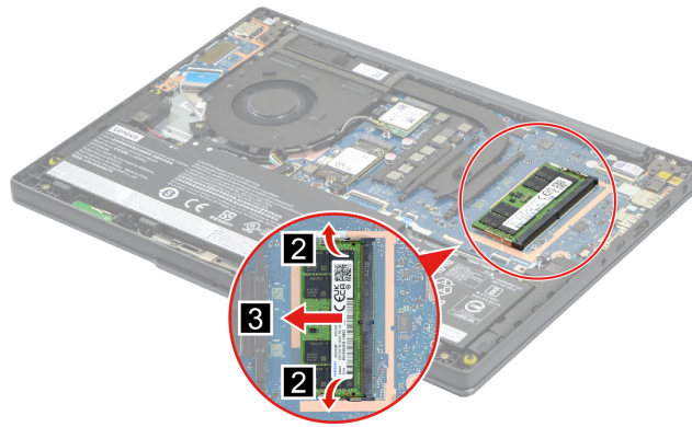
Figure 12. Remove the memory module (14-inch models/15-inch models)
