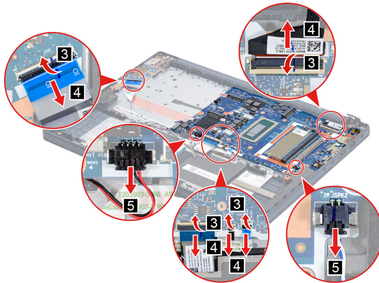
Figure 29. Disconnect cables connected to the system board
