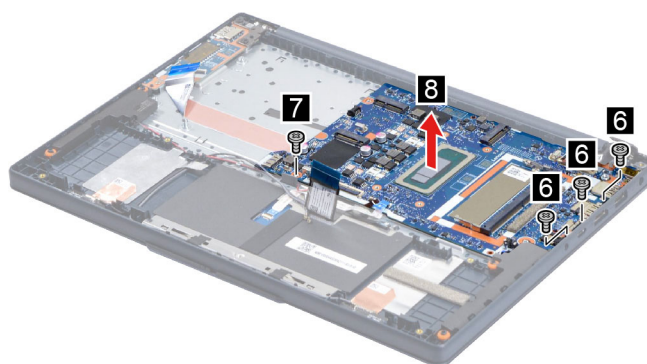
Figure 30. Remove the system board
