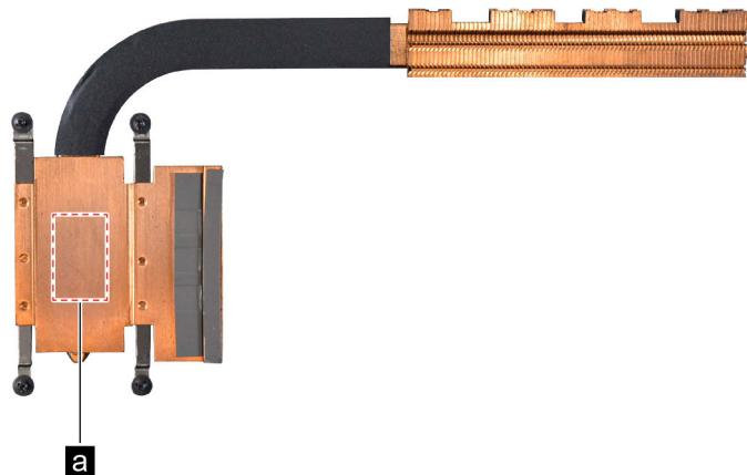
Figure 21. Areas on the heat sink where thermal interface materials should be applied
