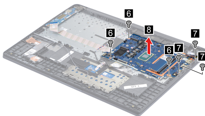
Figure 73. Remove the system board
