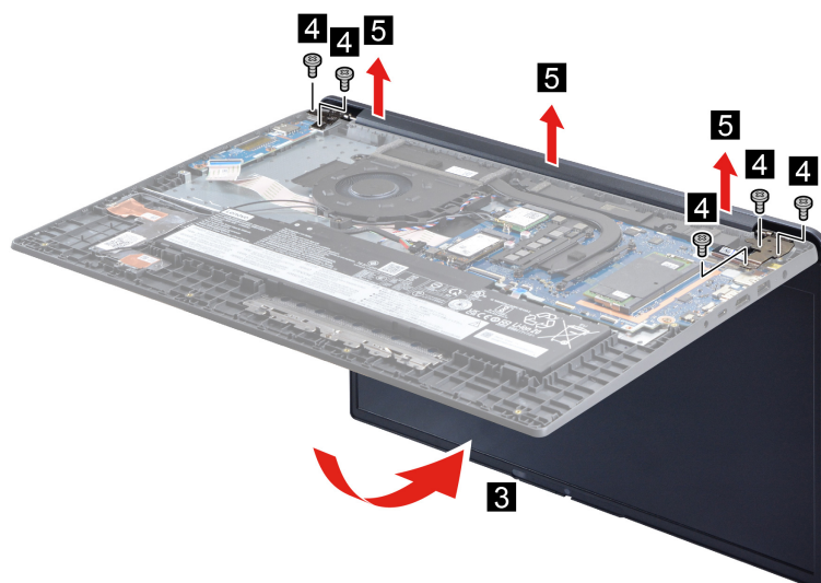
Figure 76. Remove the display assembly
