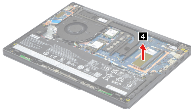
Figure 14. Remove the DDR absorber
