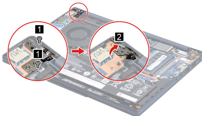
Figure 25. Flip the hinge (14-inch models)
