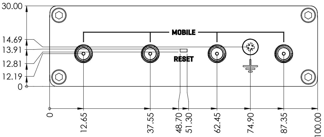
Rear view
