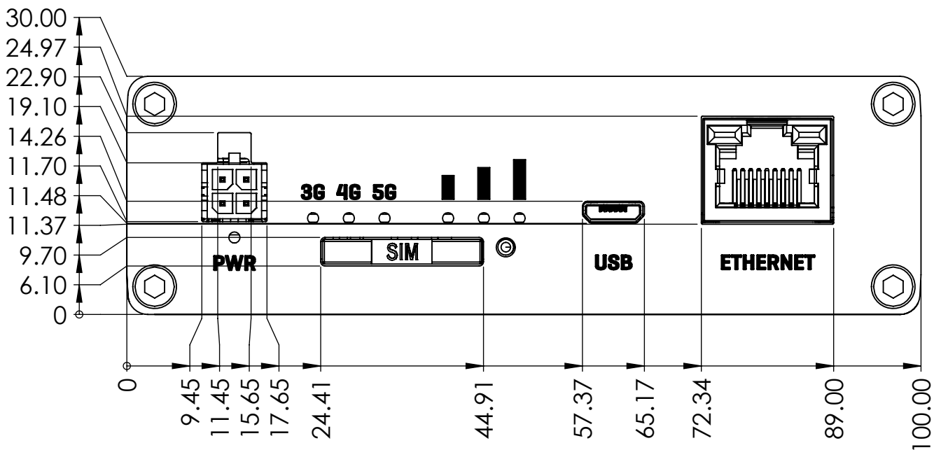
Front view
