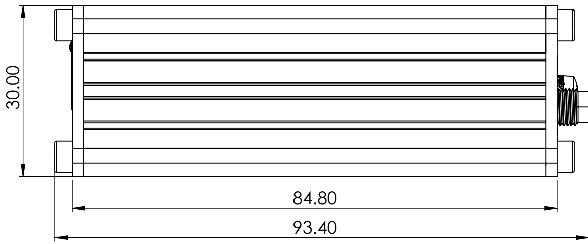
Right view
