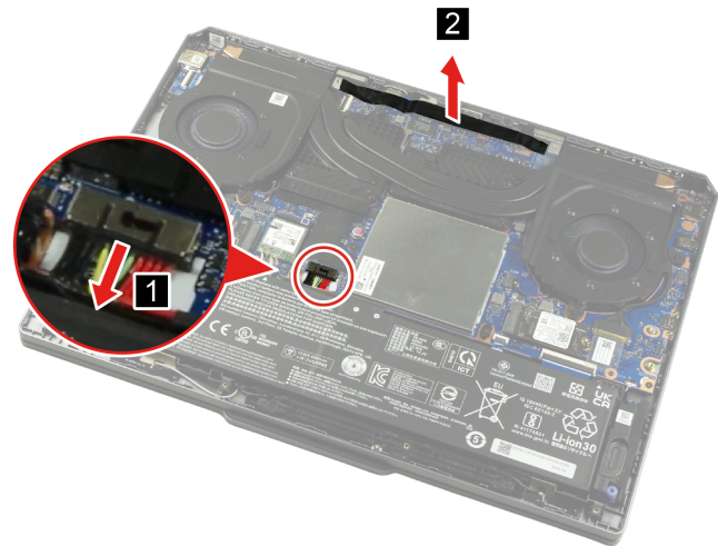
Figure 12. Disconnect the battery pack and peel off the tape
