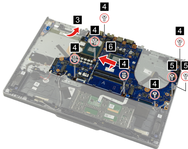
Figure 28. Remove the system board
