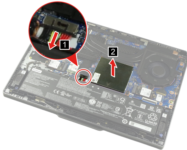
Figure 10. Remove the memory shielding
