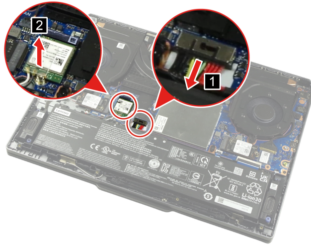
Figure 5. Remove the Wi-Fi card mylar
