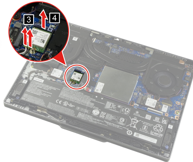
Figure 6. Remove the Wi-Fi card thermal pad
