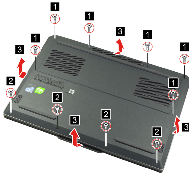
Figure 1. Remove ten screws and the lower case
