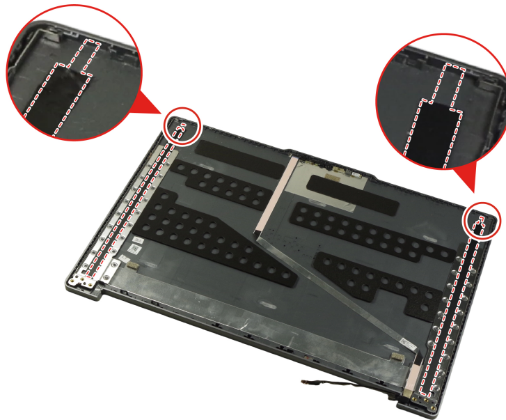
Figure 39. The locations of the stretch-release tapes
