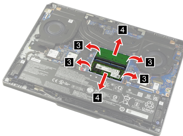
Figure 11. Remove the memory module
