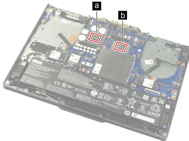
Figure 25. Areas on the system board where thermal interface materials are applied
