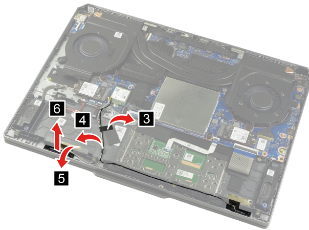
Figure 16. Remove the auxiliary antenna
