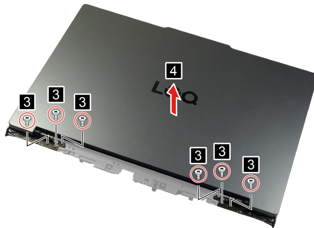
Figure 33. Remove six screws and remove the LCD module
