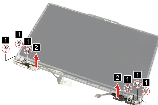
Figure 36. Remove the hinges
