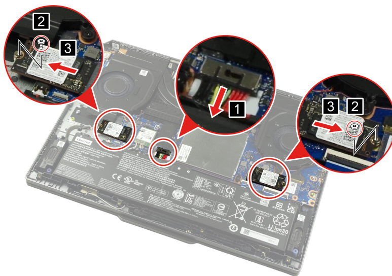
Figure 8. Remove the 2242 solid-state drives
