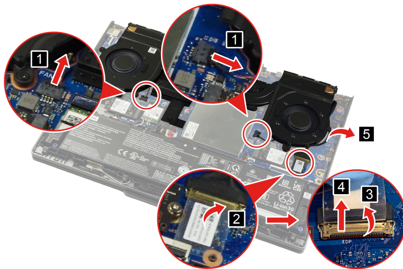
Figure 22. Disconnect the fans and the EDP cable
