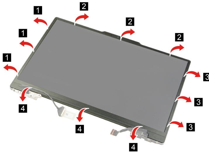
Figure 34. Remove the LCD bezel
