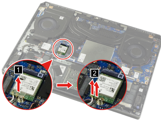
Figure 15. Detach the main and auxiliary antenna cable connectors
