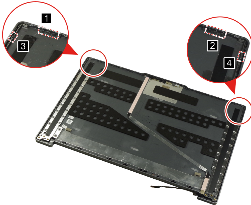
Figure 40. The locations where the rubber pads should be adhered
