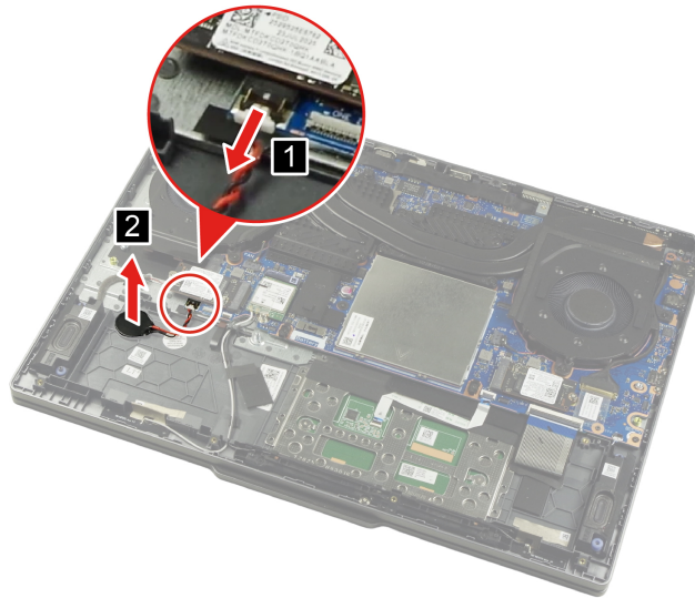
Figure 19. Remove the CMOS battery
