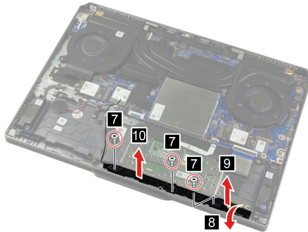
Figure 17. Remove the touchpad support bracket and main antenna
