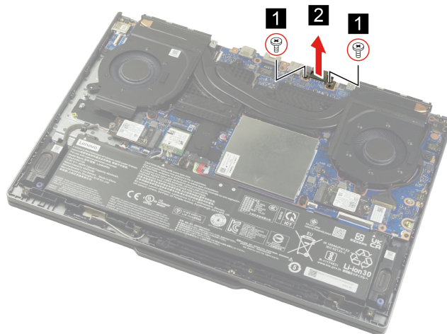
Figure 21. Remove the DC-in bracket
