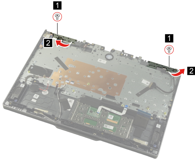
Figure 32. Remove two screws and peel off the cables
