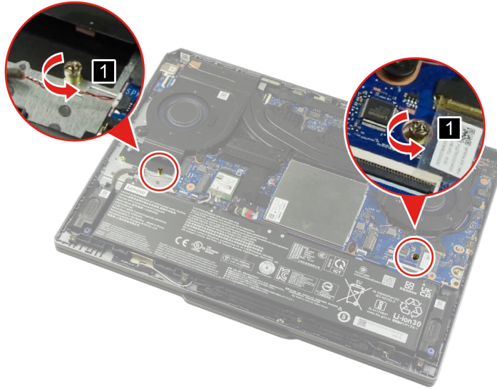
Figure 9. Remove the SSD nuts
