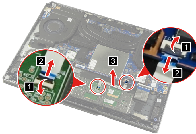
Figure 20. Remove the touchpad cable
