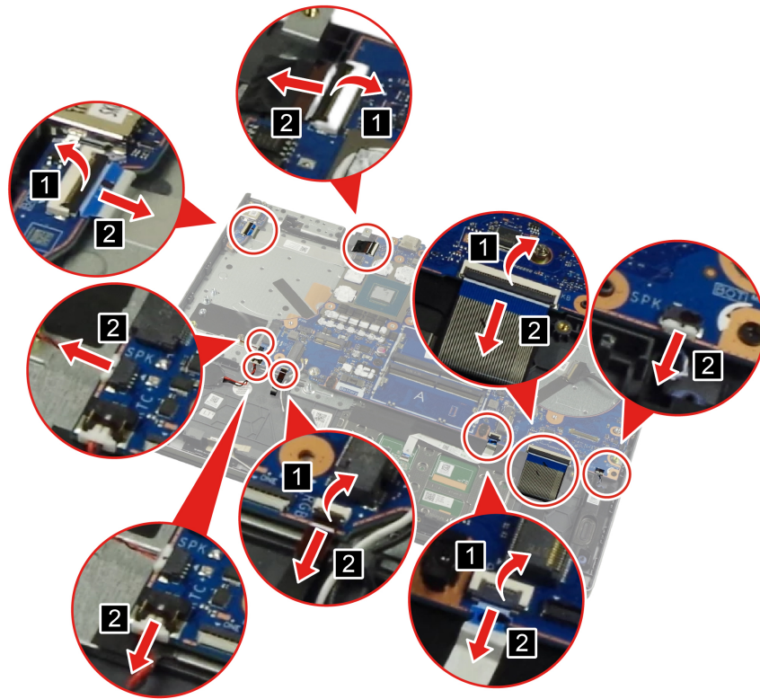
Figure 27. Disconnect the cables connected to the system board
