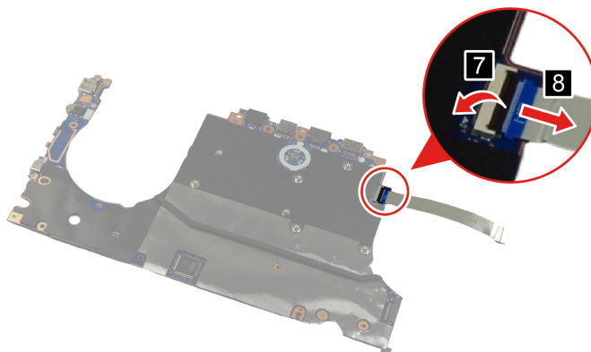
Figure 29. Disconnect the I/O board cable from the system board
