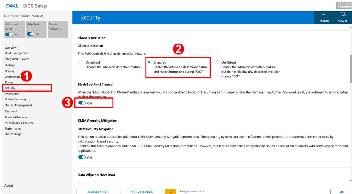
Abbildung 77. Block Boot Until Cleared
