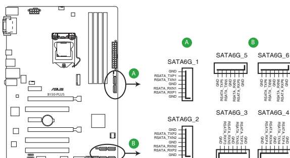
B150-PLUS Intel® SATA 6.0Gb/s connectors
