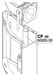
JBL CristalProfi m greenline Outlet pipe
