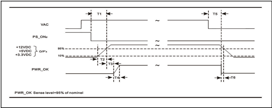
Figure 1. Power Supply Timing
