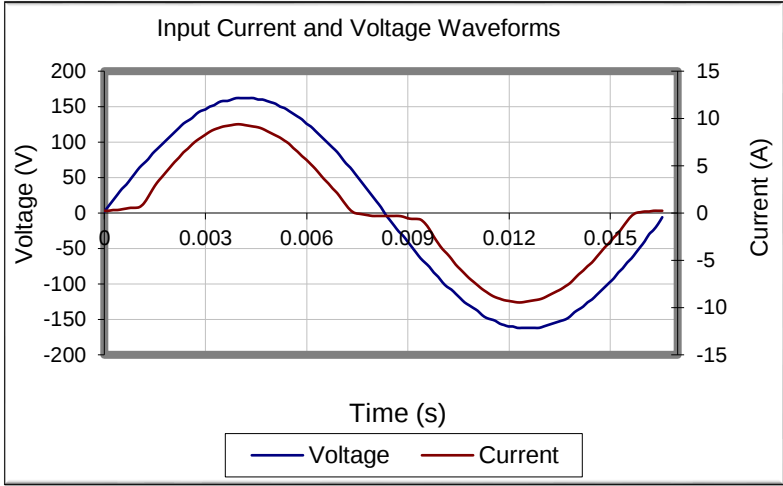
Input AC Current Waveform (ITHD = 30.83%, 50% Load)
