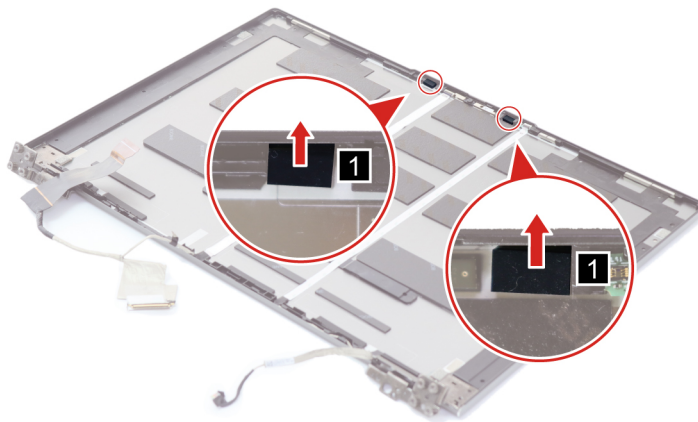
Figure 47. Remove the camera rubbers
