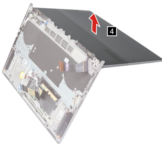
Figure 33. Remove the LCD module
