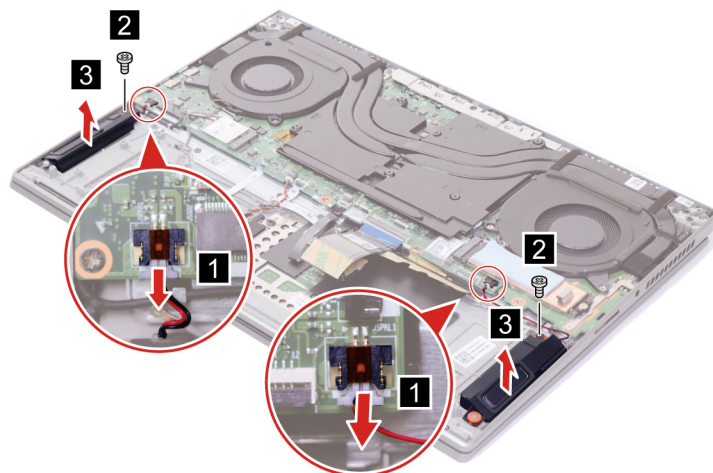
Figure 24. Disconnect cables and remove the speakers
