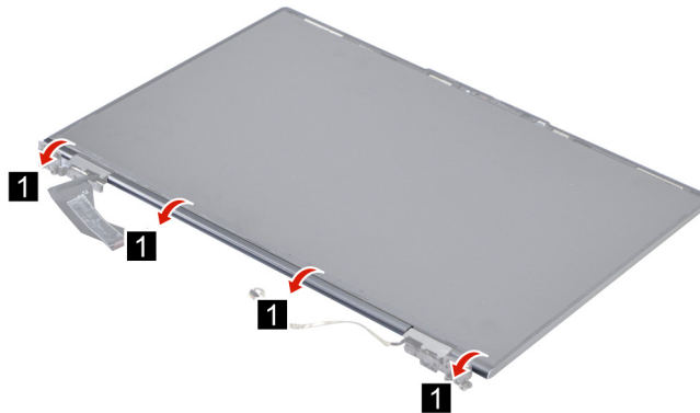
Figure 35. Remove the hinge covers
