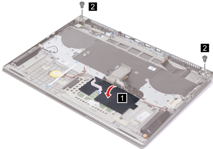
Figure 29. Peel back the touchpad board mylar and then remove two screws
