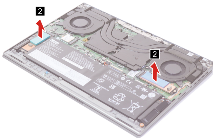
Figure 6. Remove the SSD Thermal pads
