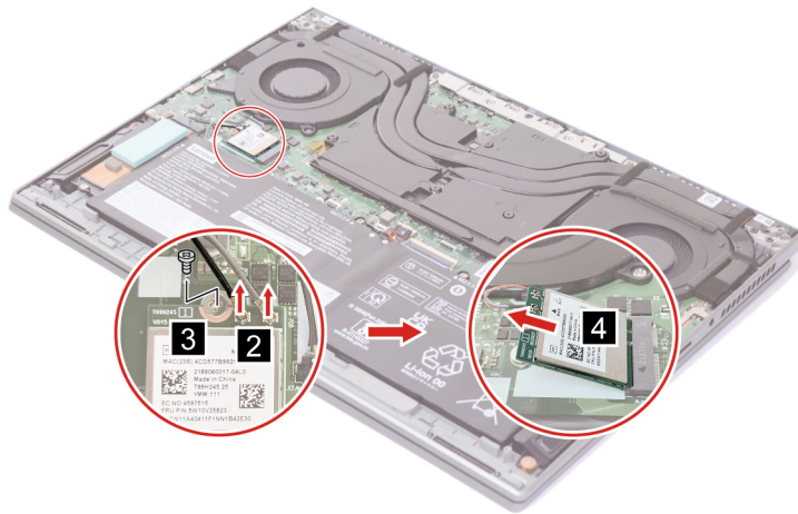
Figure 12. Remove the Wi-Fi card
