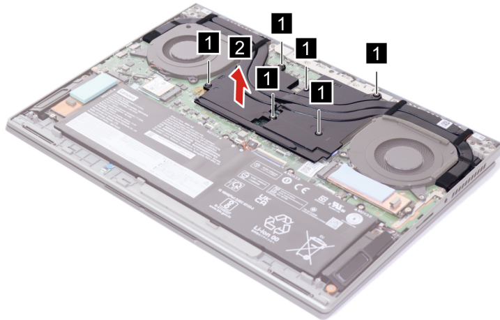
Figure 14. Loosen six screws and then remove the heat sink
