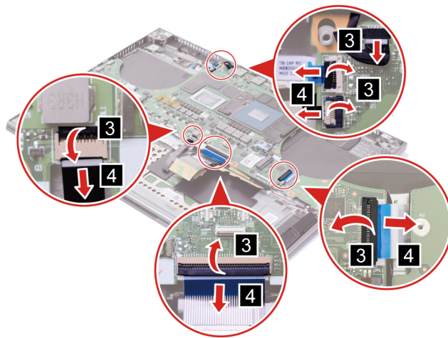
Figure 27. Disconnect cables
