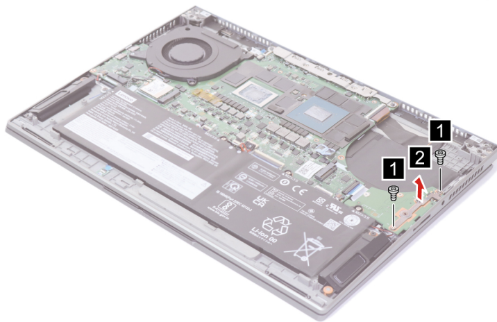
Figure 18. Remove the SSD bracket
