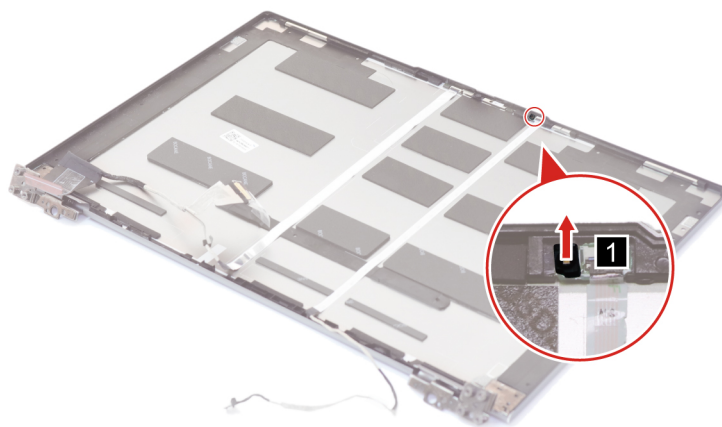
Figure 38. Remove the ambient light sensor (ALS) board rubber
