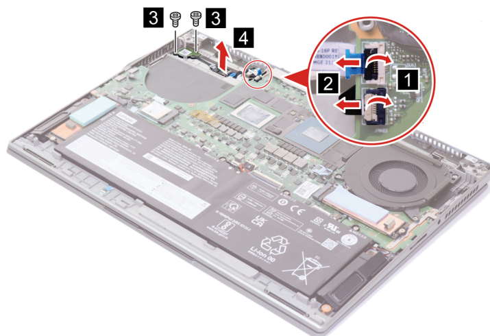
Figure 16. Disconnect the fingerprint reader board cable and remove the fingerprint reader board with cable
