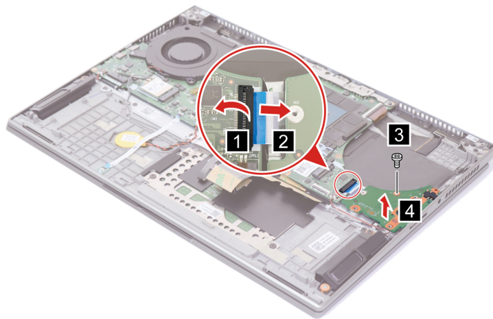
Figure 19. Disconnect the USB board cable and remove the USB board with cable
