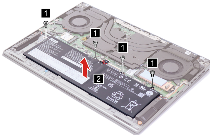
Figure 10. Remove four screws and the battery pack
