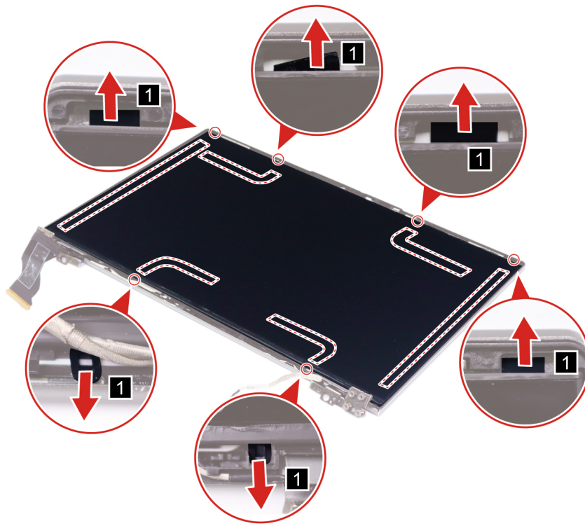
Figure 36. Remove the six pieces of removable tape with tweezers
