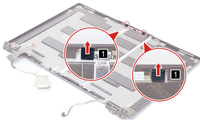
Figure 43. Remove the microphone rubbers
