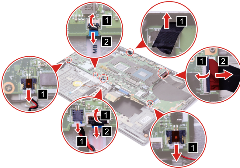
Figure 26. Disconnect cables
