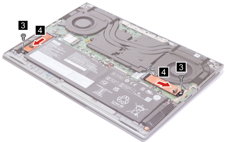
Figure 7. Remove two screws and the SSD modules
