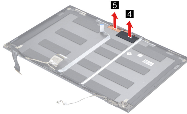
Figure 46. Remove the sponge and then remove the IR camera CU foil
