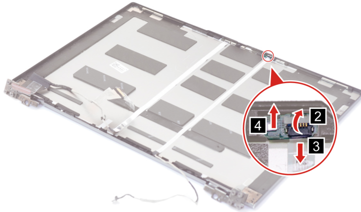
Figure 39. Remove the ambient light sensor (ALS) board
