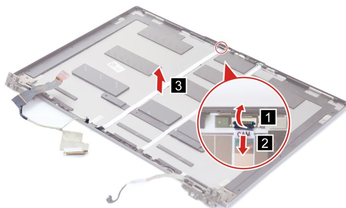
Figure 42. Remove the EDP cable
