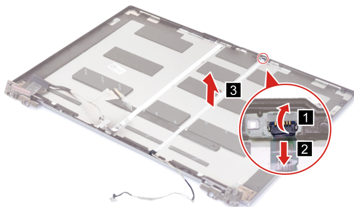
Figure 40. Remove the ambient light sensor (ALS) board cable
