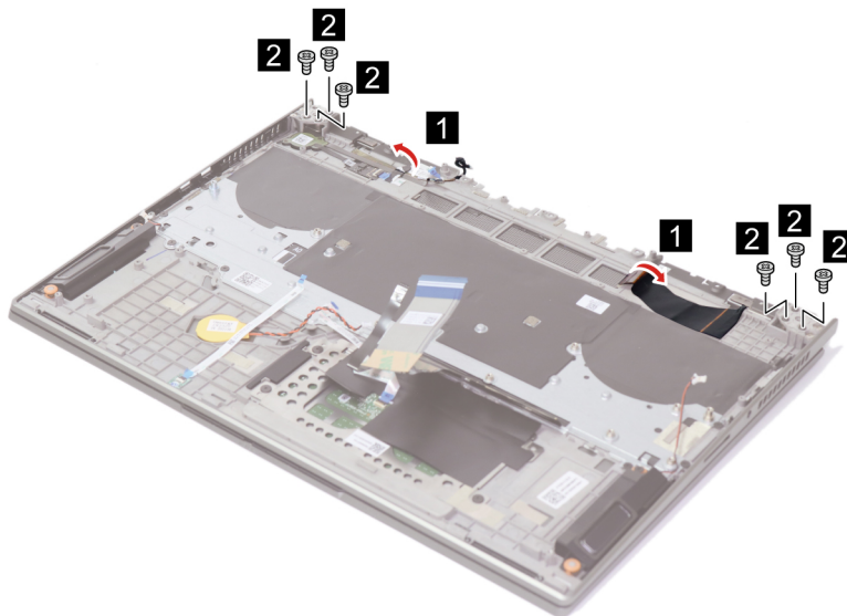
Figure 31. Remove six screws
