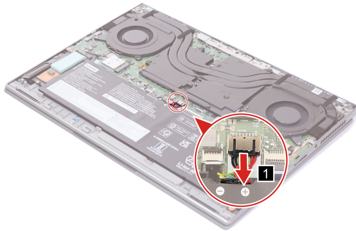
Figure 5. Disconnect the battery pack cable
