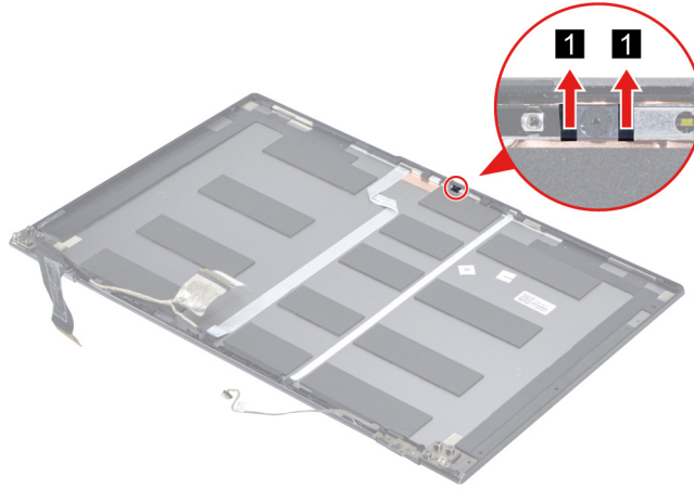
Figure 44. Remove the IR camera sponges
