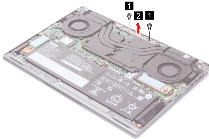
Figure 13. Remove two screws and the DC-in bracket
