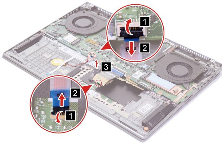
Figure 25. Remove the touchpad board cable
