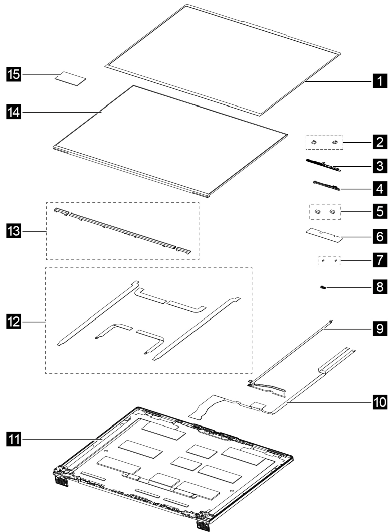
Figure 2. LCD module — exploded view
