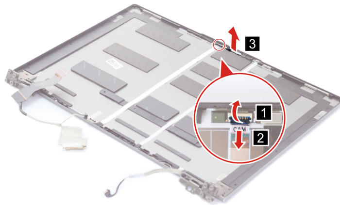
Figure 45. Remove the camera
