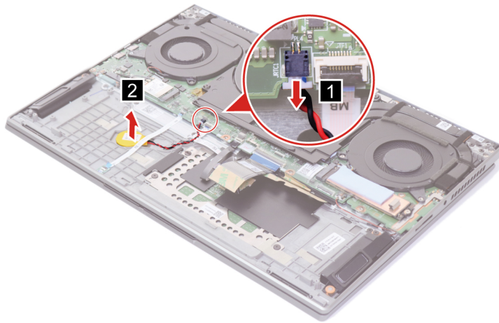
Figure 23. Disconnect the CMOS battery cable and remove the CMOS battery
