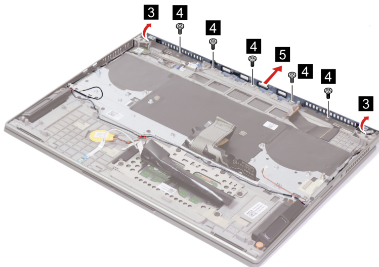
Figure 30. Remove the strip cover
