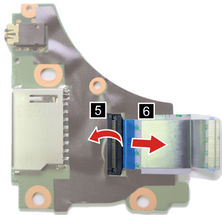
Figure 20. Separate the USB board cable from the USB board
