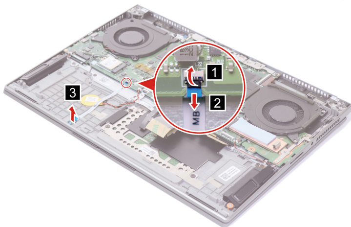
Figure 21. Disconnect the hall sensor board cable and remove the hall sensor board with cable
