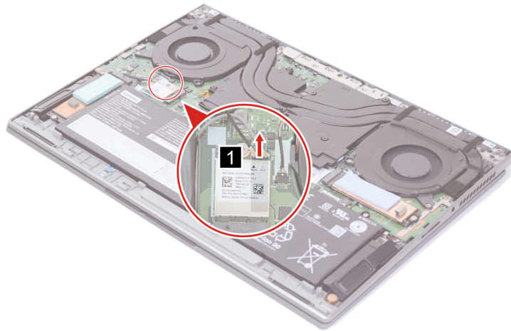
Figure 11. Peel off the Wi-Fi card mylar
