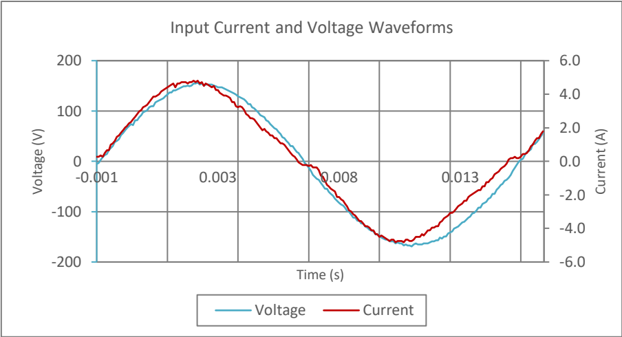
Input AC Current Waveform (ITHD = 8.82%, 50% Load)
