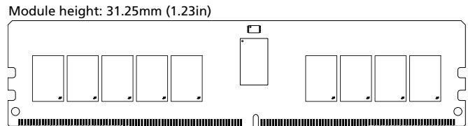
Figure 1: 288-Pin RDIMM (MO-309, R/C-E1, R/C-E2)
