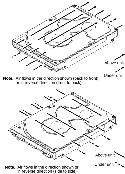
Figure 10. Air flow
