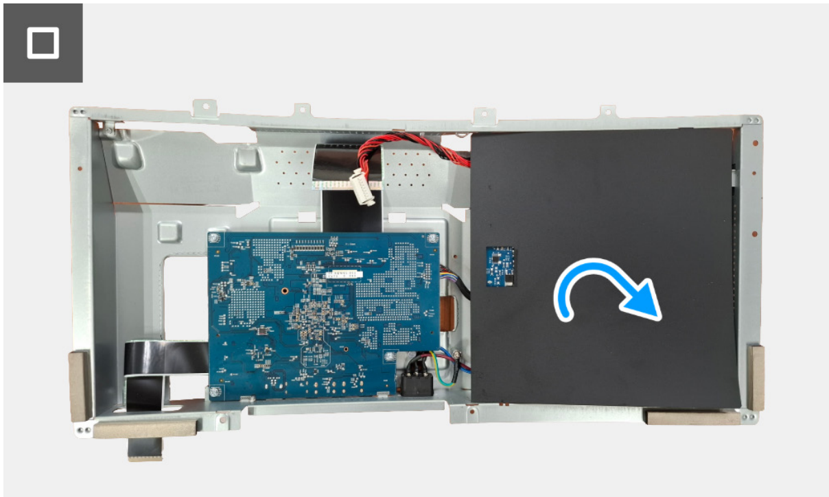
Figure 25. Installing the interface board
