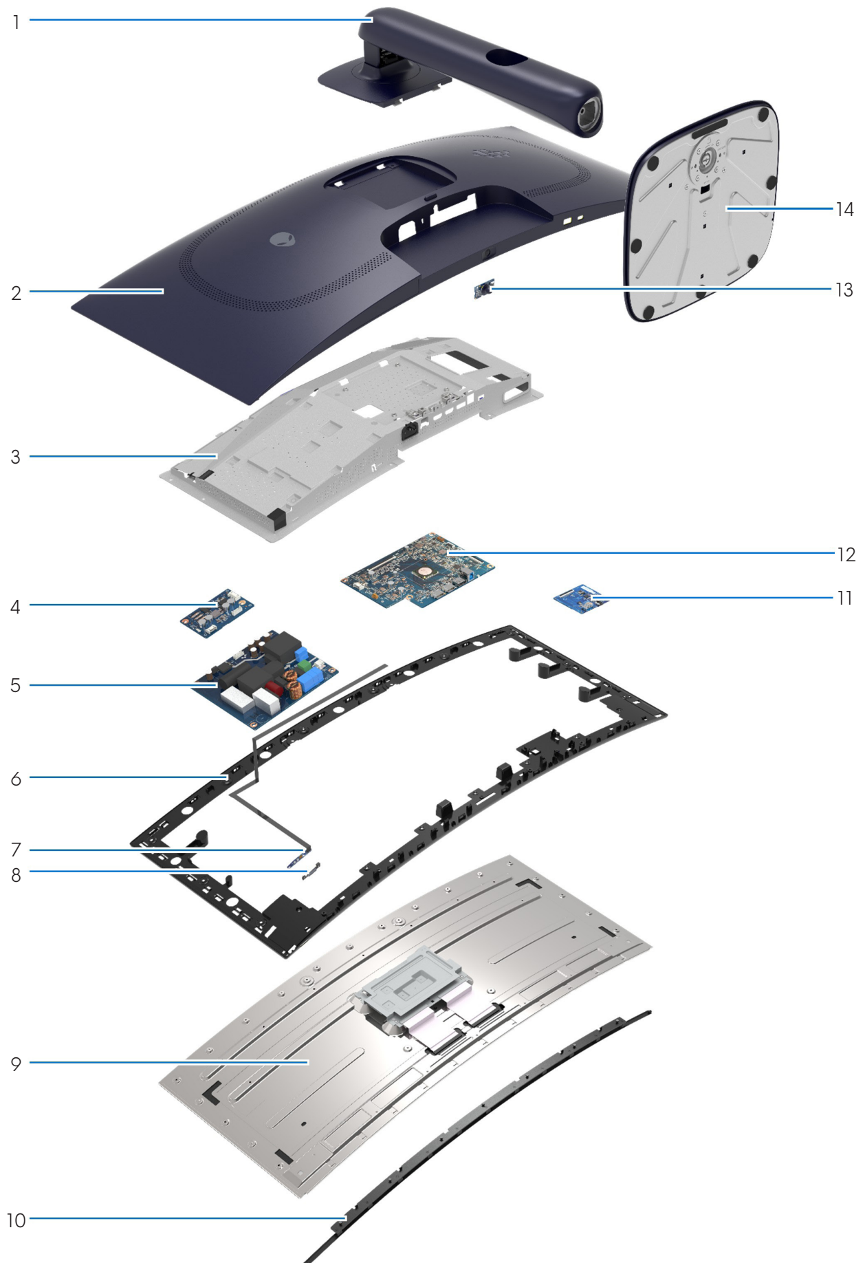
Figure 5. Major components of AW3426DW monitor
