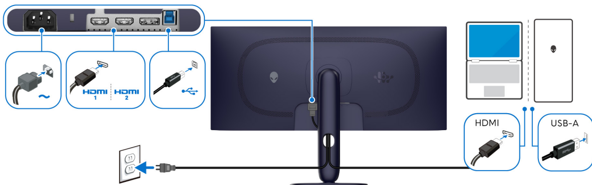
Figure 9. HDMI connection
