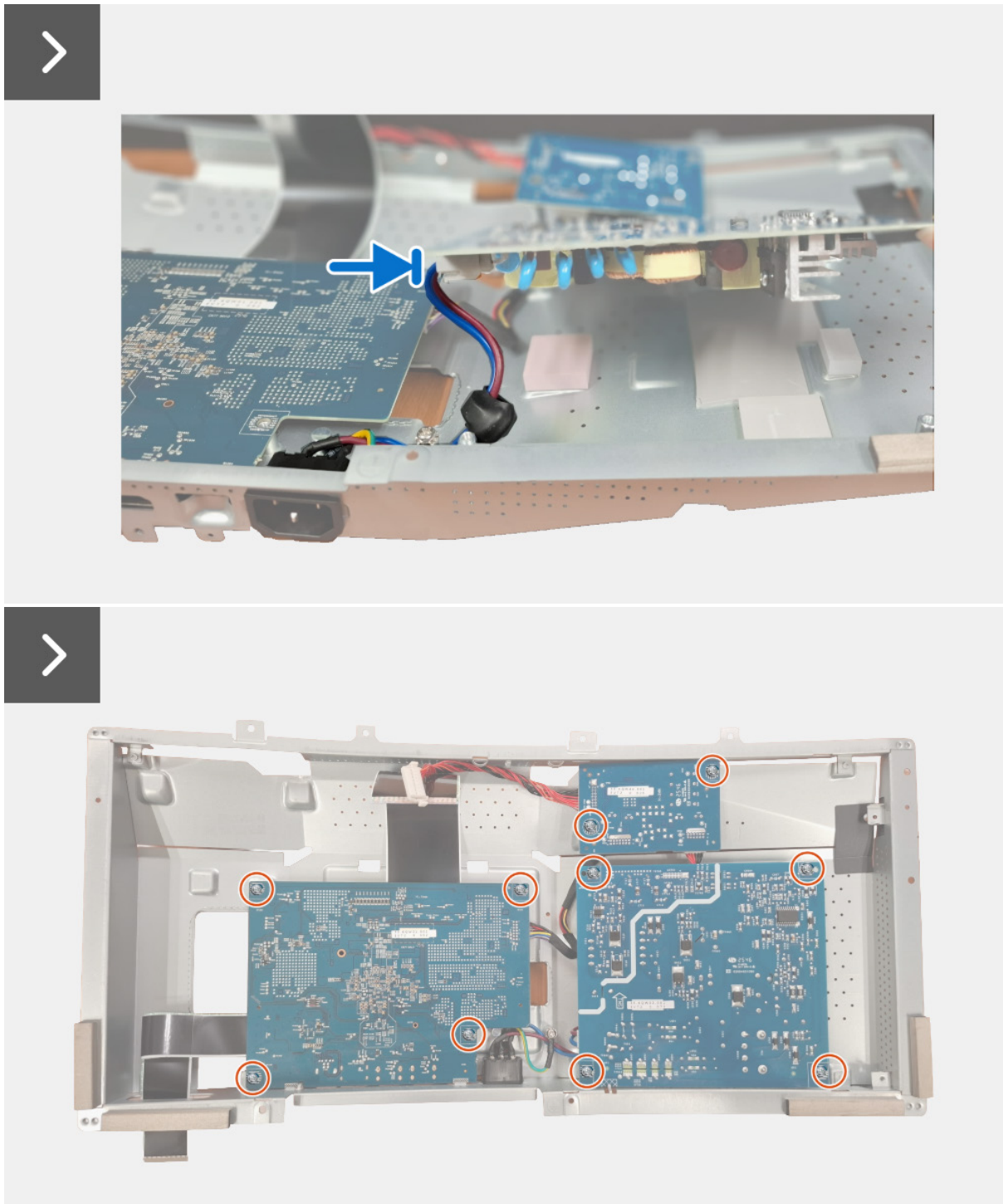
Figure 24. Installing the interface board
