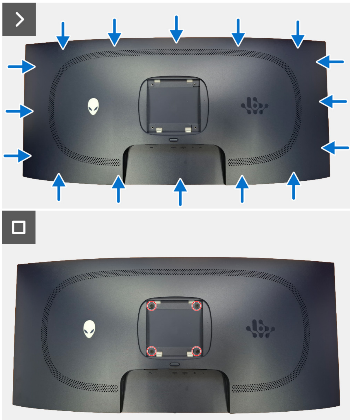
Figure 16. Installing the back cover
