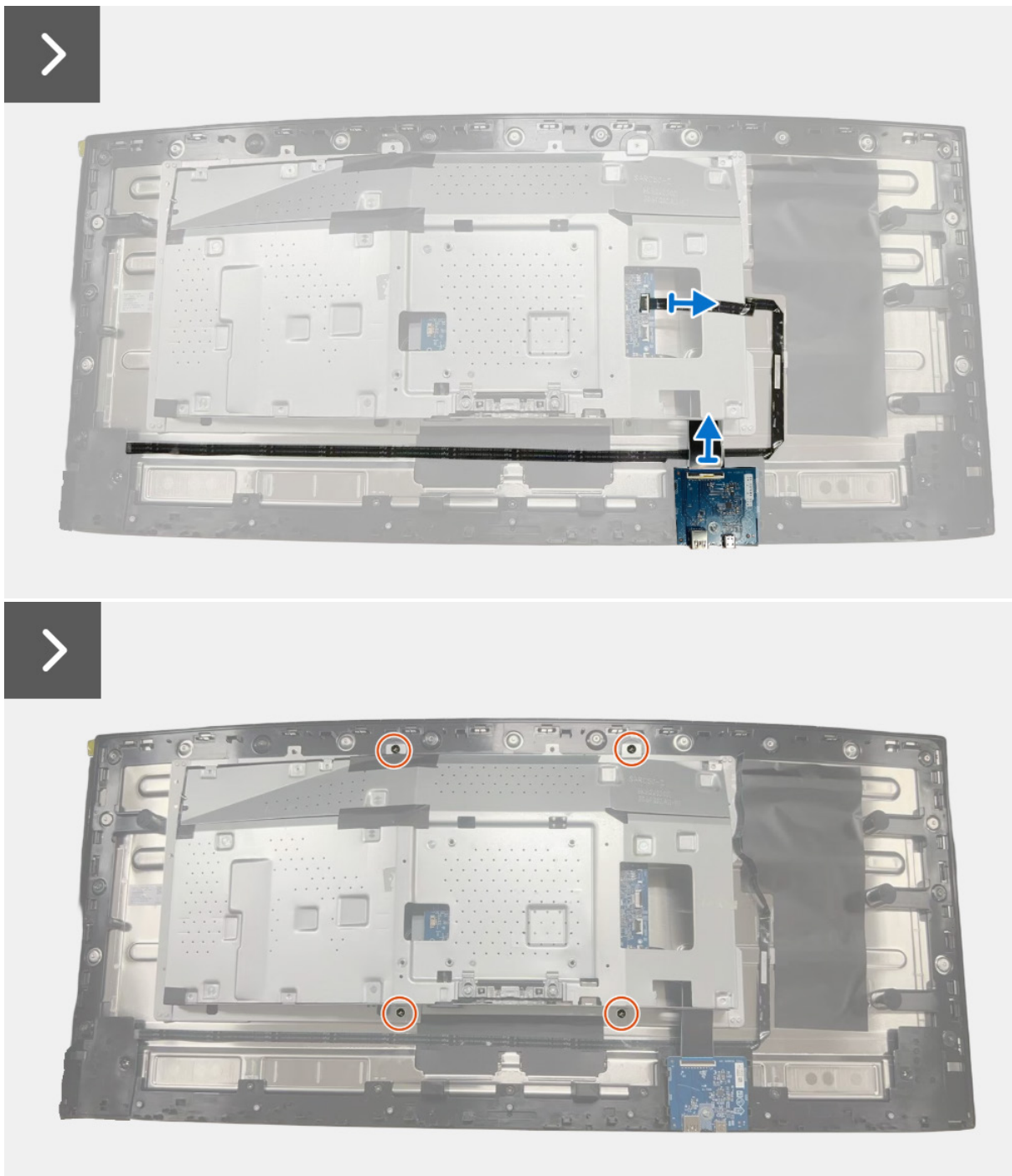
Figure 17. Removing the metal shield
