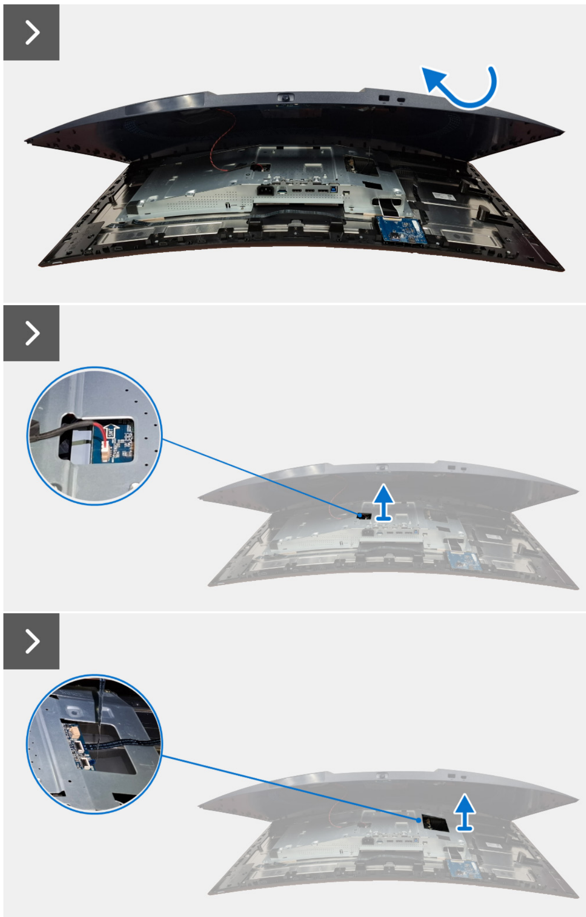
Figure 13. Removing the back cover
