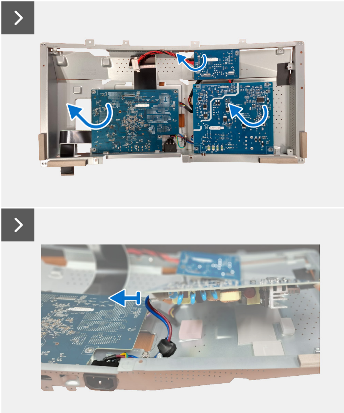
Figure 22. Removing the interface board
