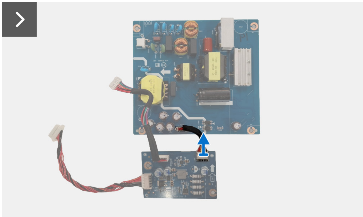
Figure 26. Removing the power board
