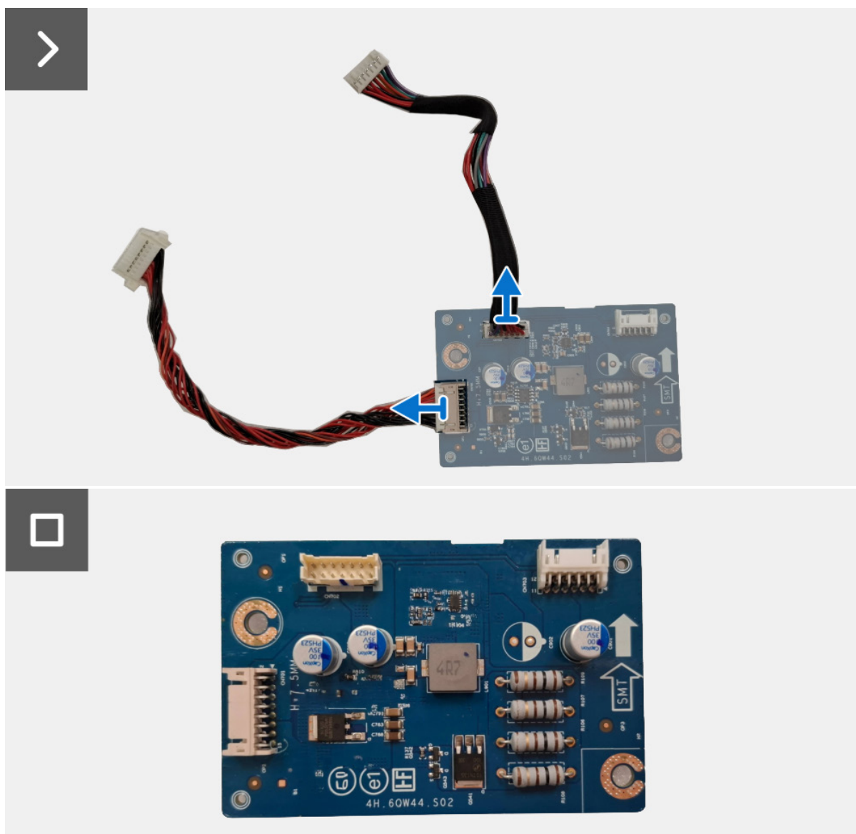
Figure 29. Removing the DC-DC board
