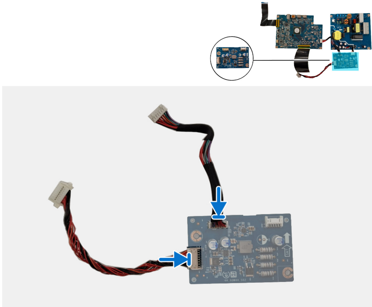
Figure 30. Installing the DC-DC board
