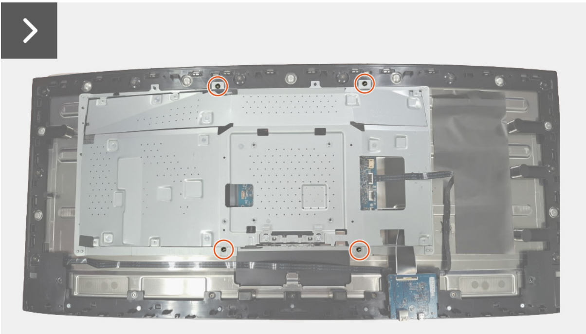
Figure 19. Installing the metal shield
