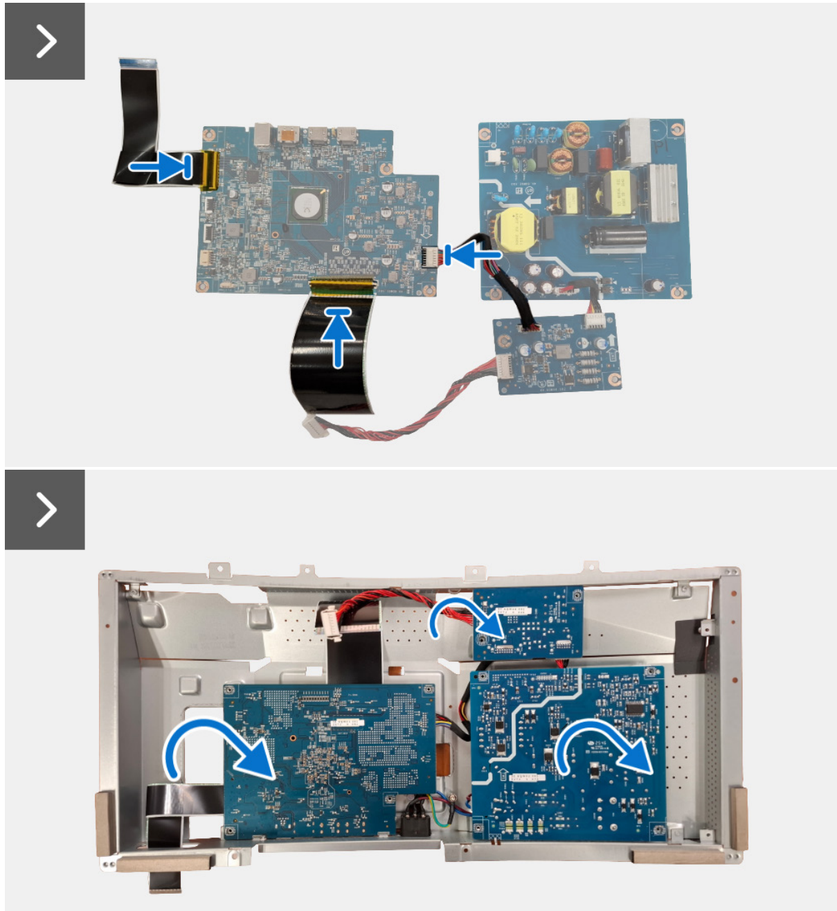
Figure 23. Installing the interface board
