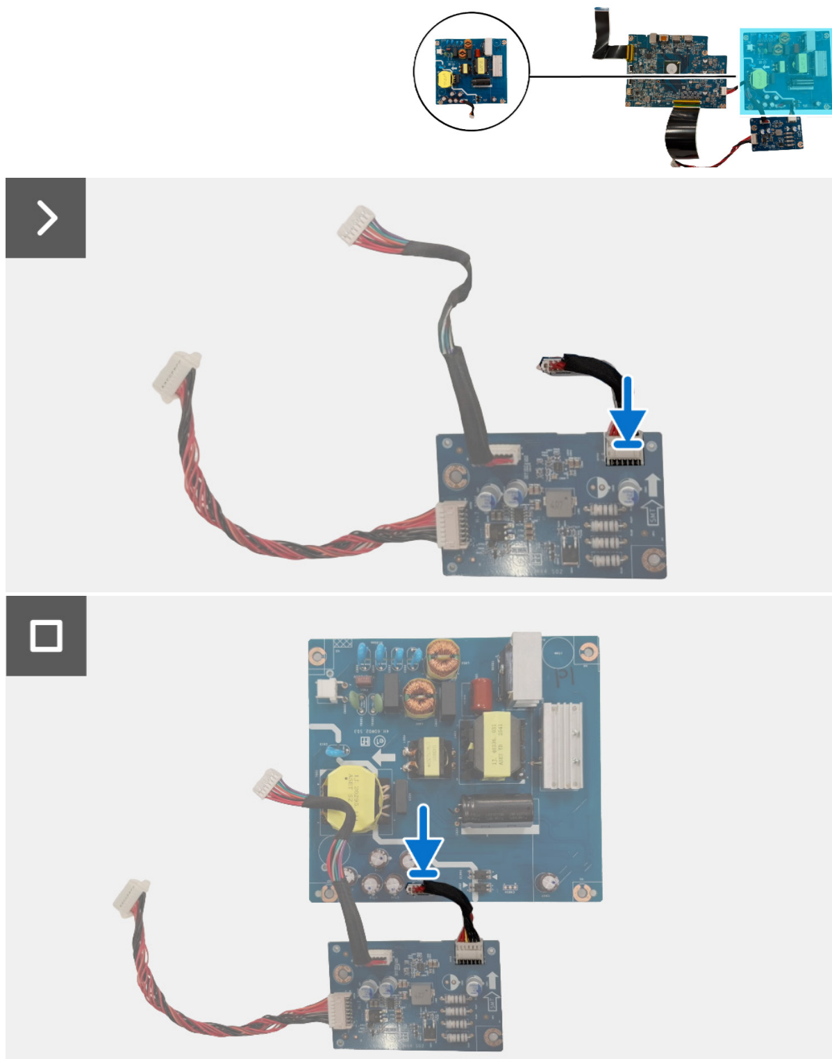
Figure 28. Installing the power board
