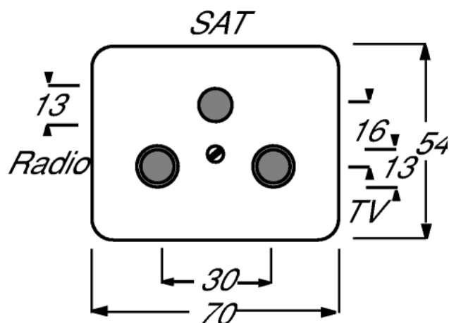
Cover plate with 3 connections for SAT /Audio /TV, 1743-03-...
