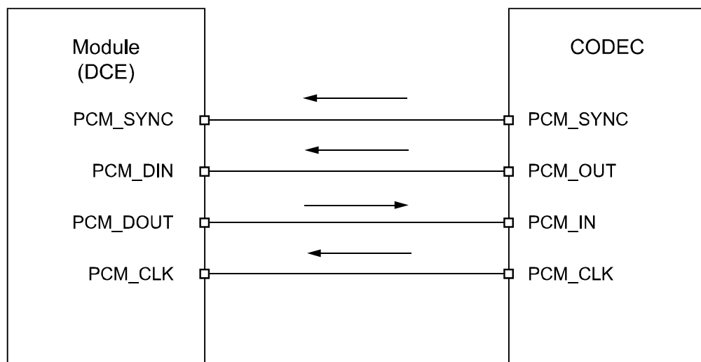
Figure 3-15 Circuit diagram of the interface of the PCM (ME909s Mini PCIe module is used as PCM slave)
