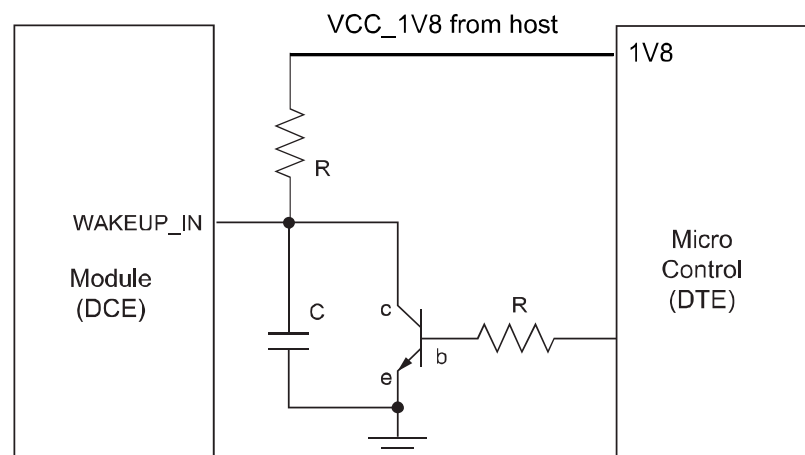
Figure 3-5 Connections of the WAKEUP_IN pin
