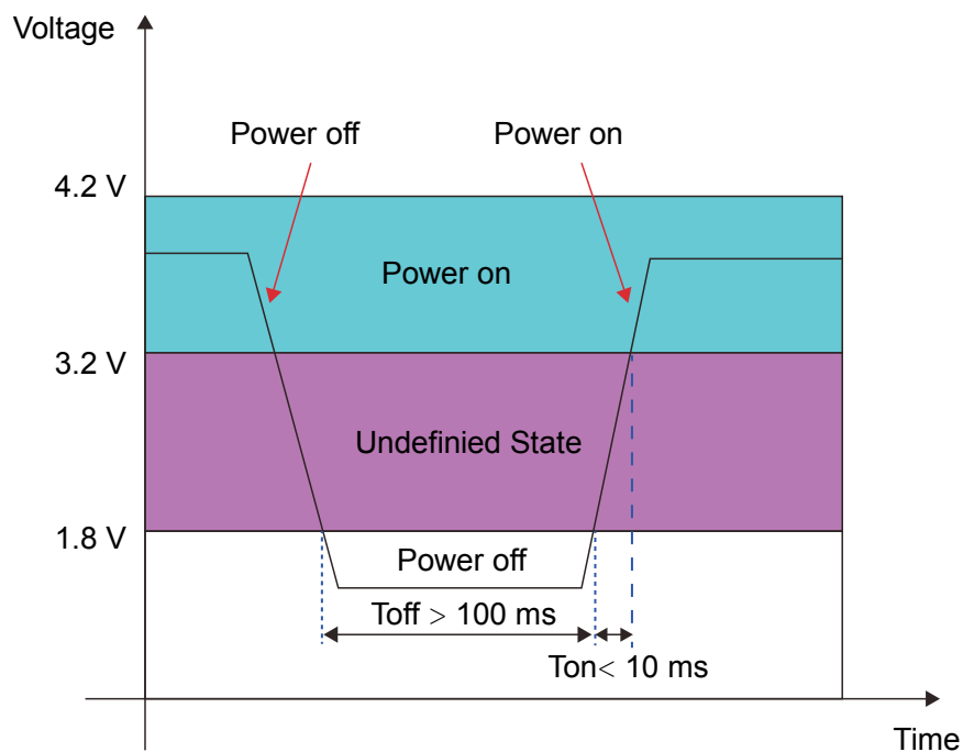
Figure 3-3 Power supply time sequence for power cycling
