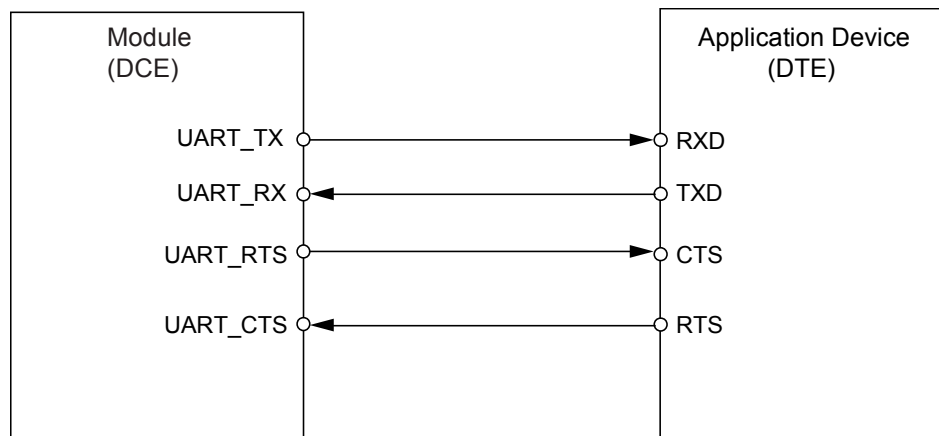
Figure 3-9 Connection of the UART interface in the ME909s Mini PCIe module (DCE) with the host (DTE)
