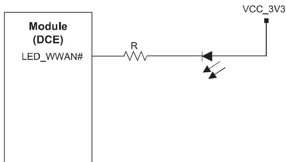
Figure 3-8 Driving circuit
