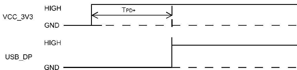
Figure 3-2 Power on timing sequence
