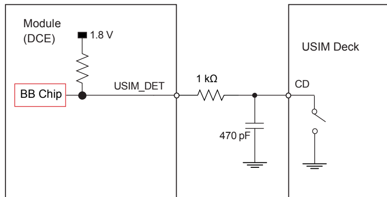
Figure 3-11 Connections of the USIM_DET pin
