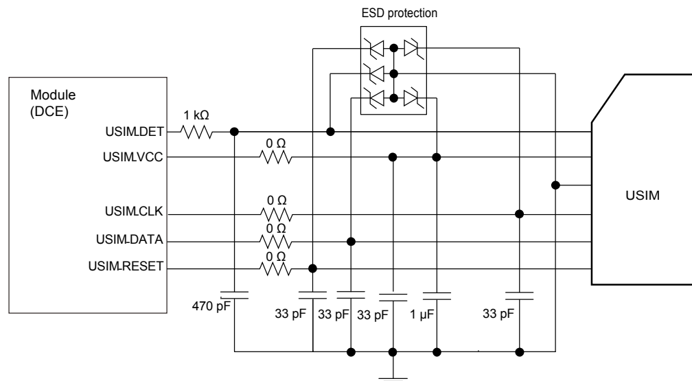
Figure 3-13 Circuit of the USIM card interface
