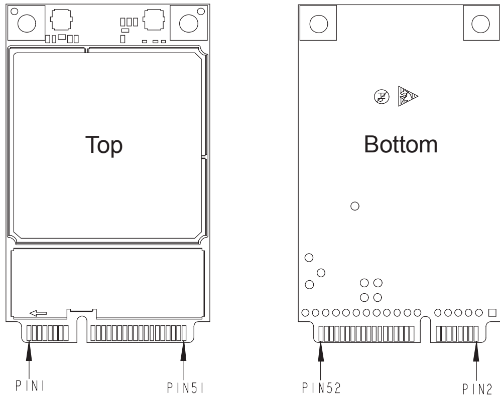
Figure 3-1 Sequence of Mini PCIe interface
