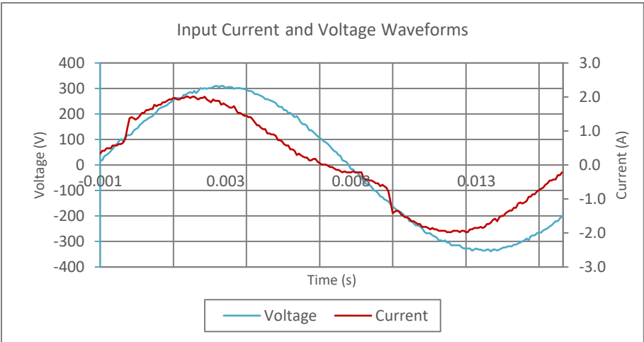
Input AC Current Waveform (ITHD = 17.47%, 50% Load)
